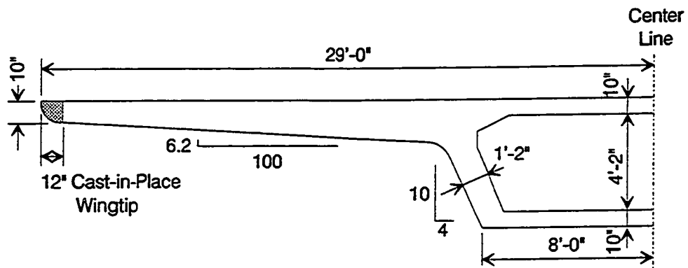
b) Typical Type III Segment Spans A43 and A44
