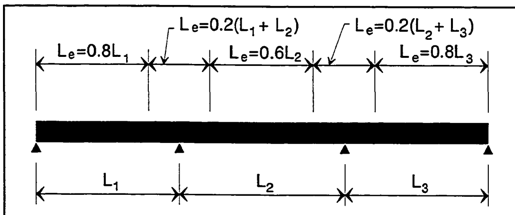
Figure 5.8 Effective span lengths for Ontario Bridge Code effective flange width calculations.
