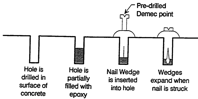
Figure 3.14 Modified Demec attachment system.
