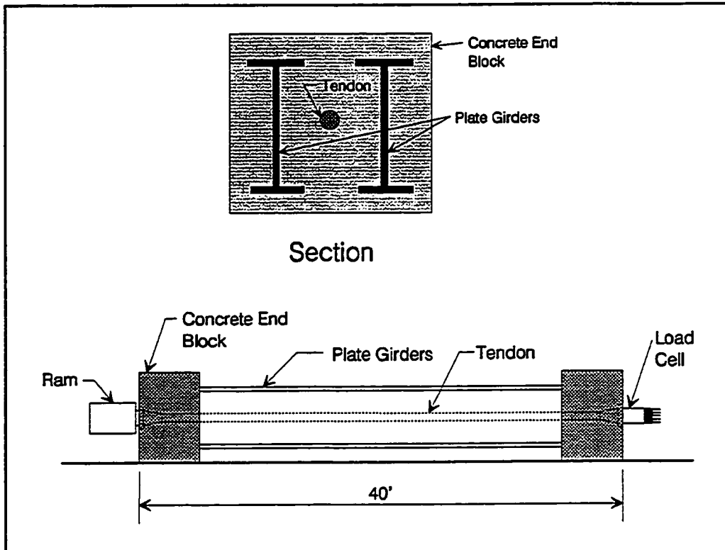
Figure 4.2 Austin Bridge and Road bench test frame.
