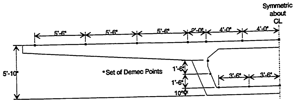
Spans A43 and A44 Demec Point Layout
