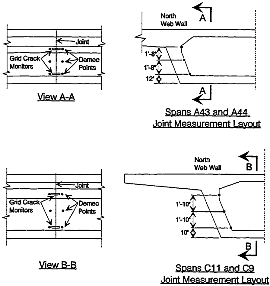
Figure 3.25 a) Joint movement instrumentation layouts.
