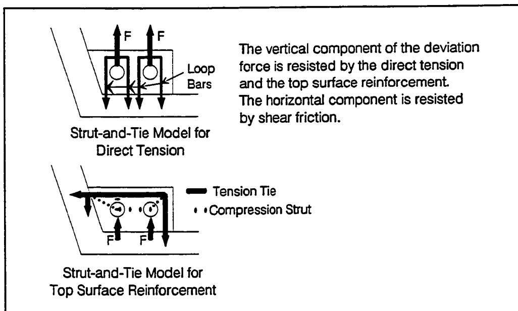
Figure 9.2 Beaupre et al. strut-and-tie model for deviator.
