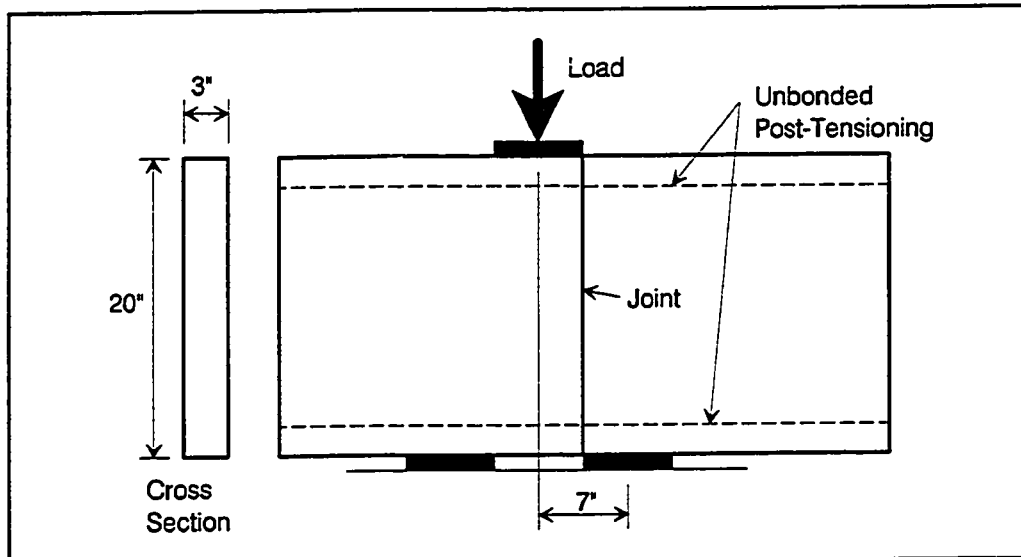
Figure 7.5 Specimens of Koseki and Breen.
