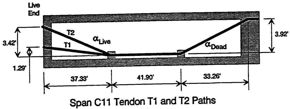
Figure 4.12 Elevation views of tendon layouts.
