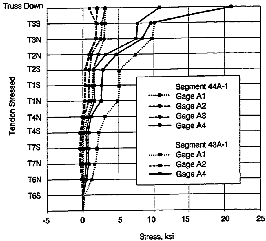
Stresses in Vertical Reinforcing Bars in Diaphragm Segments
