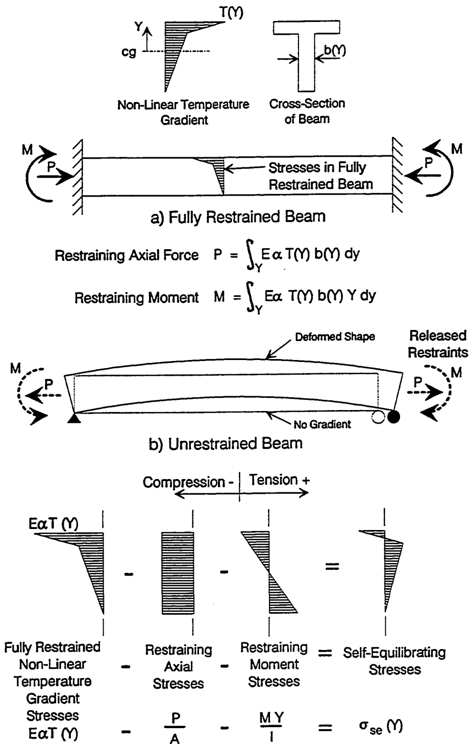
Figure 6.3 Beams subjected to non-linear gradient.
