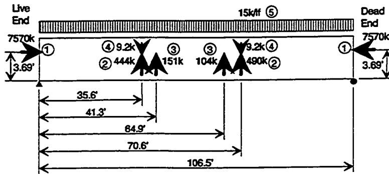
Span A44 Loading Diagram for SHLAG
