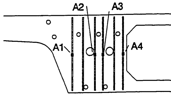
Stresses in Vertical Reinforcing Bars in Diaphragm Segments
