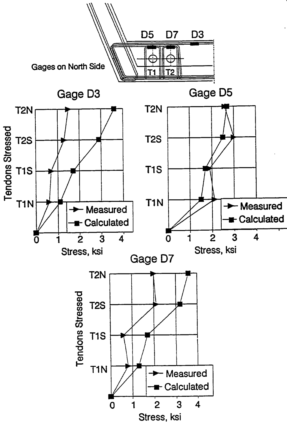
Figure 9.12 Calculated vs. measured strains in C11 deviator.
