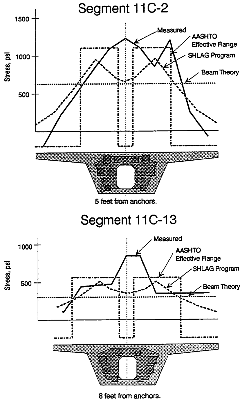
Figure 5.16 c) Top slab stress distributions, one segment from anchors.
