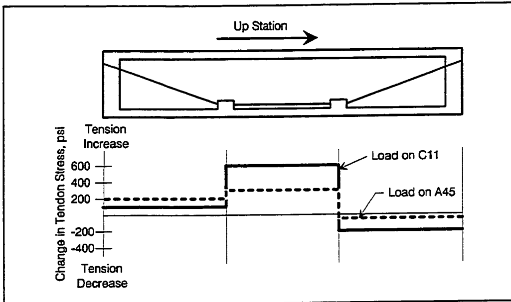
Figure 10.26 Change in tendon stress in span C11 under live loads.
