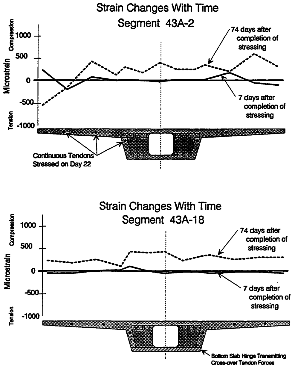
Figure 5.25 Changes in top slab strains with time.
