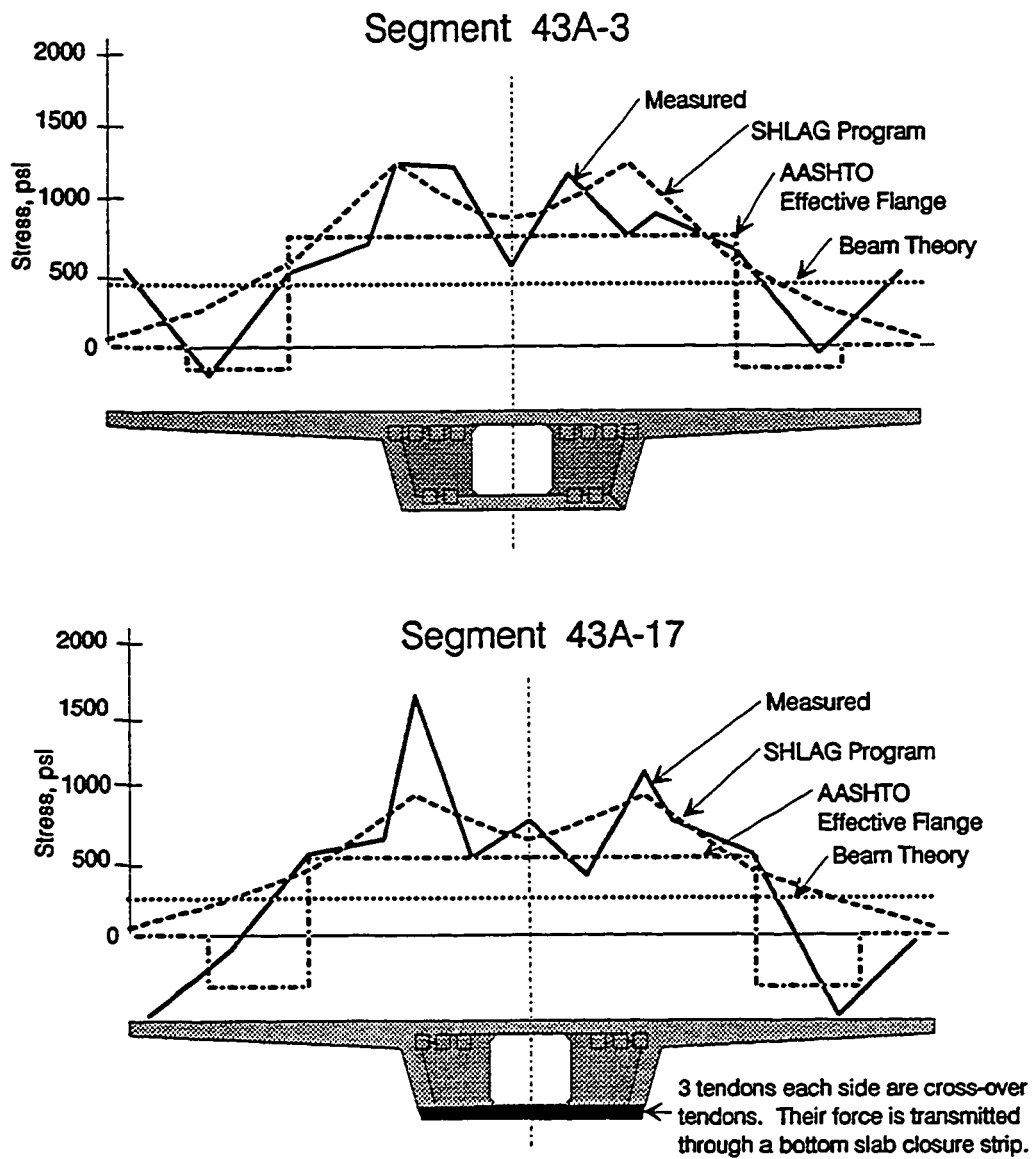
Figure 5.17 a) Top slab stress distributions, eleven feet from anchors.
