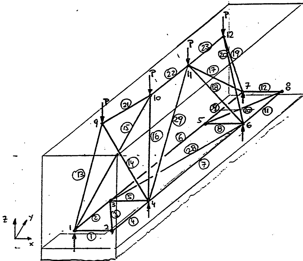
Figure 8.19 Strut-and-tie model for Washington Metro pier segments.
