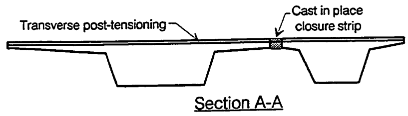
Figure 10.5 Span C11 detail
