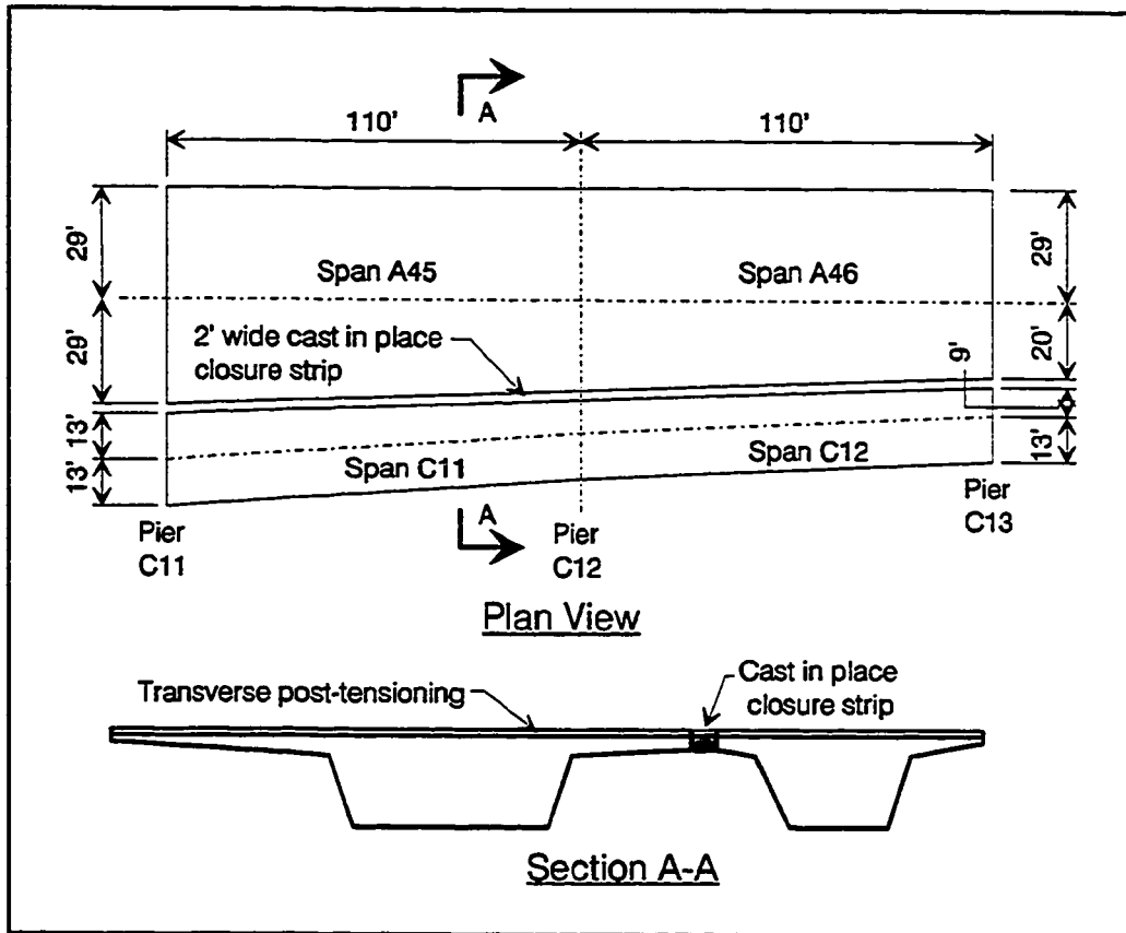
Figure 3.3 Span C11 details.
