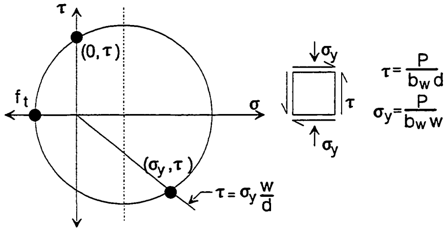
Figure 7.21 Mohr's circle description of state of stress on element near joint.
