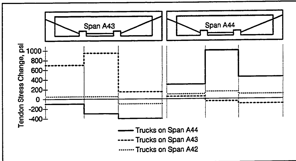
Figure 10.15 Tendon stress changes with live loads.
