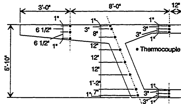
Segments 11C-4 and 11C-9 Vertical Thermocouple Layout
