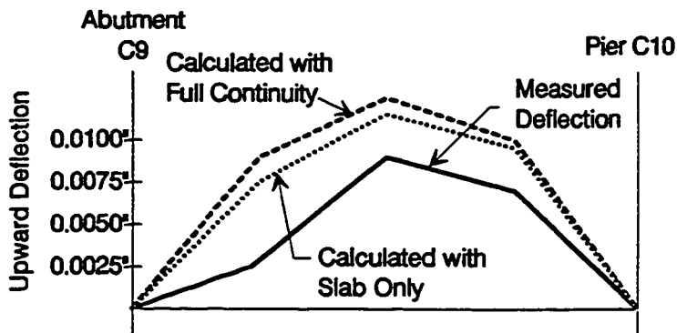
Deflections of Span C9 with Live Load on Span C10
