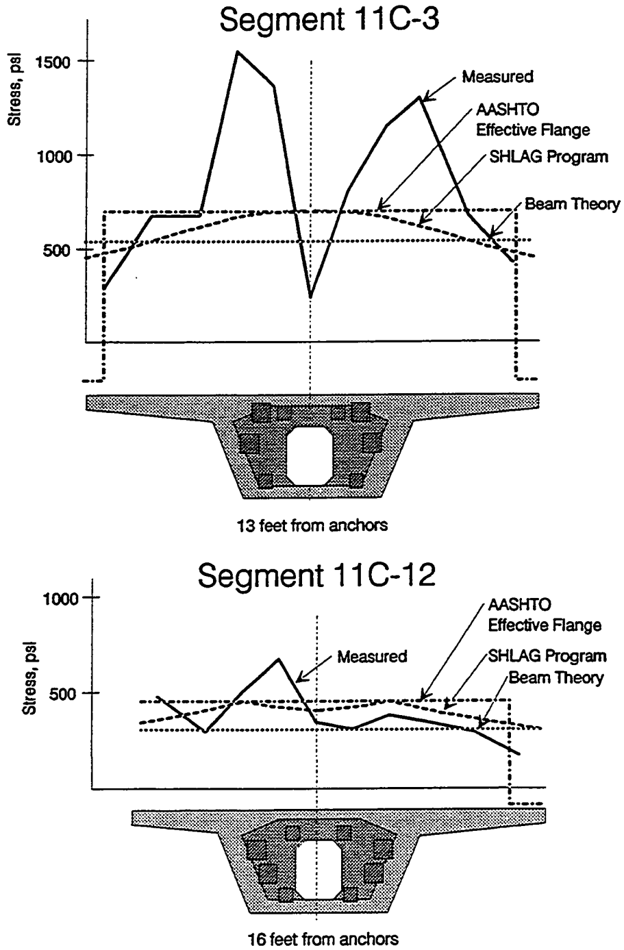
Figure 5.17 c) Top slab stress distributions, two segments from anchors.
