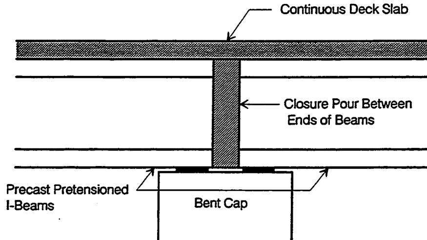
Figure 10.1 Full continuity between precast I-beams.
