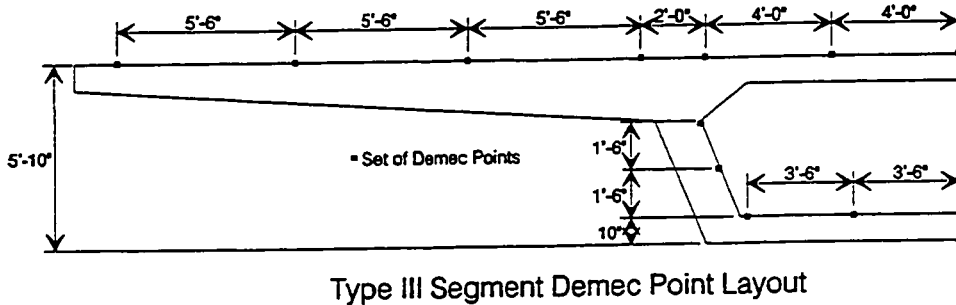
Figure 7.11 Segment Demec point layouts.
