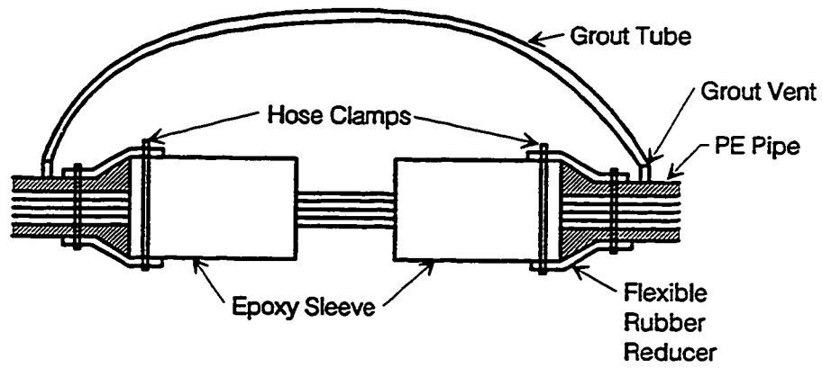
Figure 3.10 a) Grout by-pass system for Span C11.
