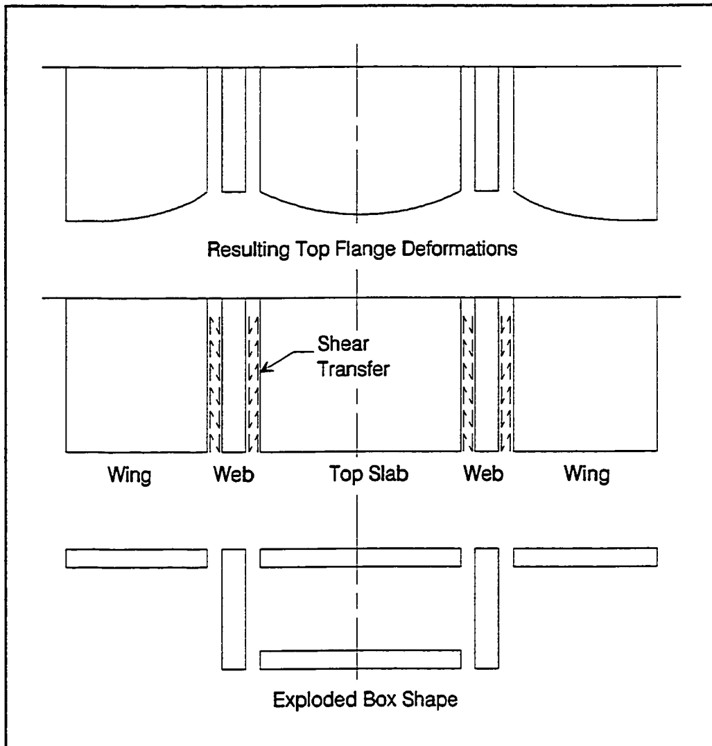
Figure 5.1 Shear lag and resulting deformations.
