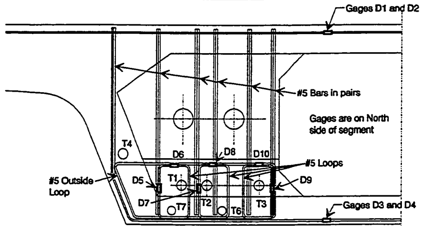
Segments 43A-7 & and 44A-7 Deviator Segment Elevation View
