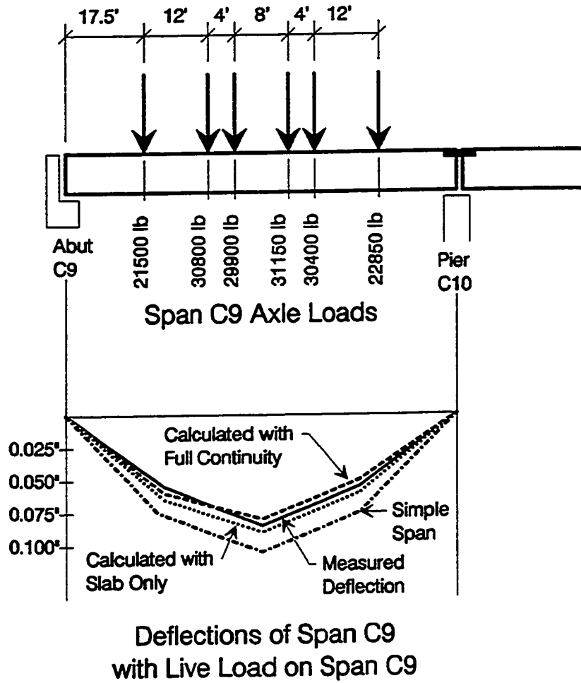
Figure 10.18 Calculated vs. actual deflections of span C9 with live load on span C9.
