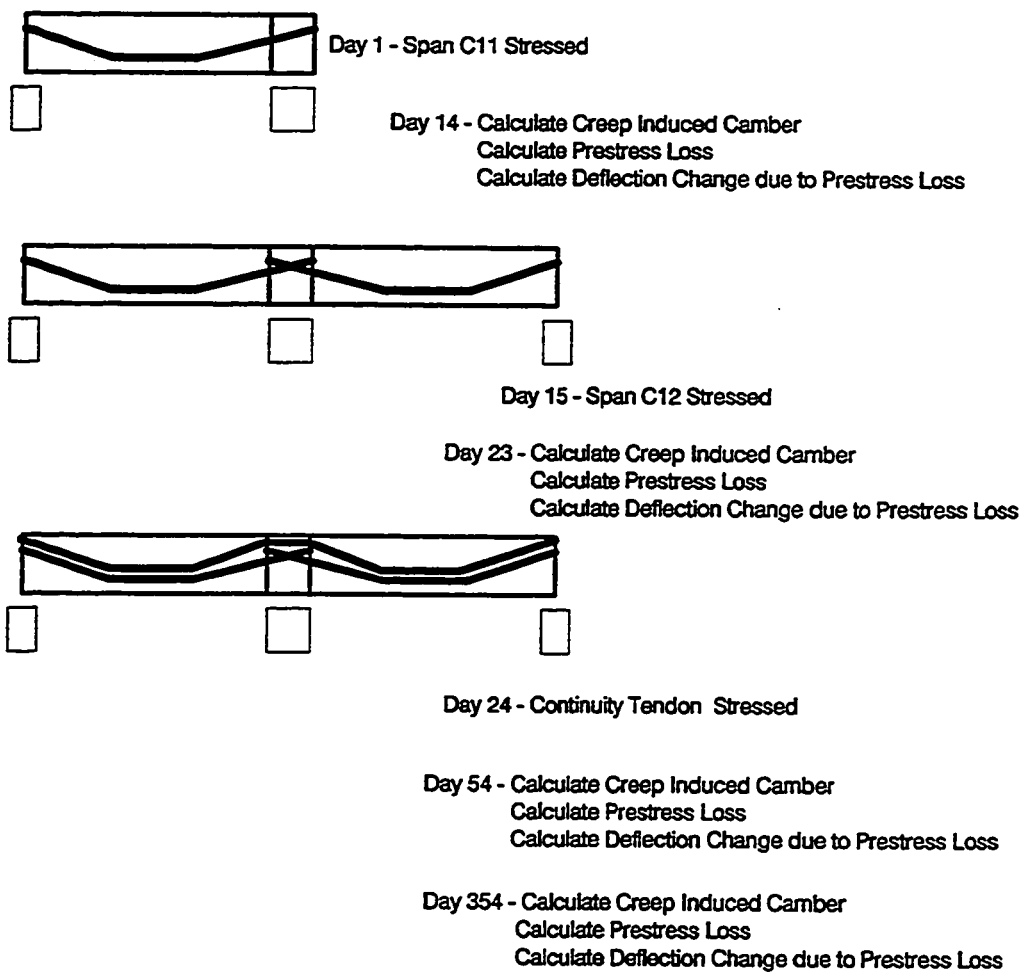
Figure 4.21 b) Erection schedule and operations of long term analysis for Spans C11.
