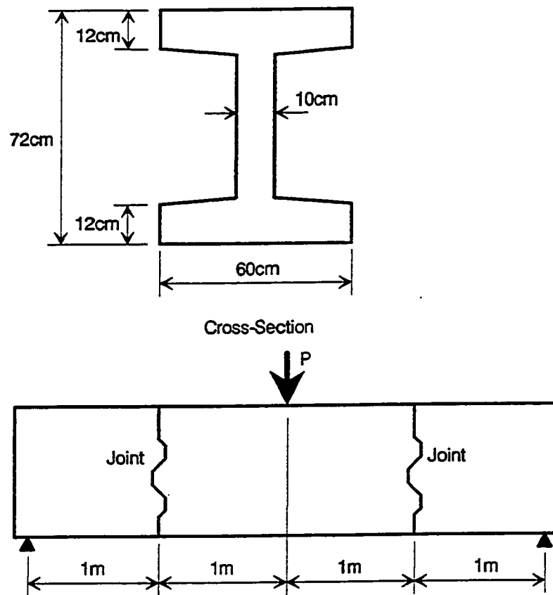
Figure 7.8 Specimens by Kordina and Weber.
