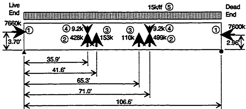
Span A43 Loading Diagram
