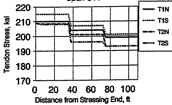
Tendon Stresses Span C11
