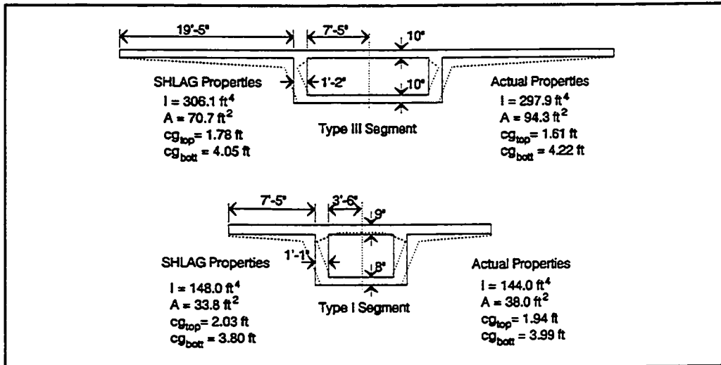
Figure 5.13 Segment properties for SHLAG program.
