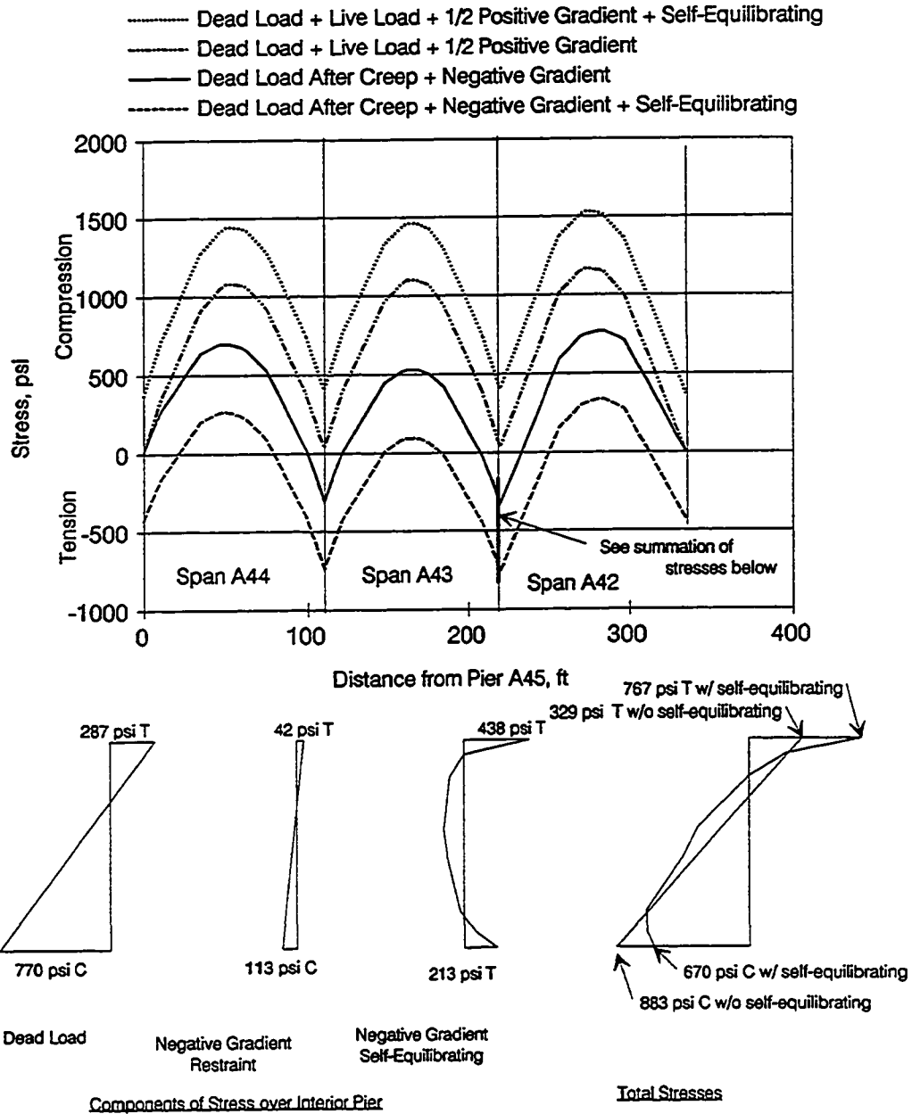
Figure 6.33 b) Comparison of top fiber stresses without prestressing, with and without self-equilibrating stresses.
