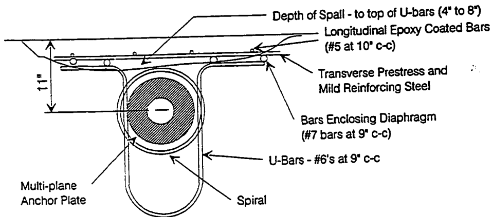
Anchorage Device and Reinforcing as Built in Expansion Joint Segments
