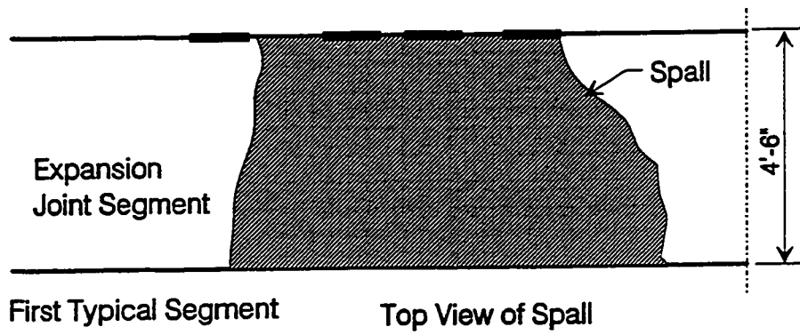
Figure 8.17 Typical spall in expansion joint segment.
