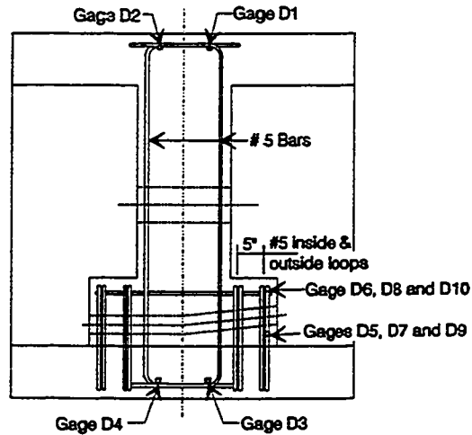
Segment 44A-7 and 43A-7 Section View
