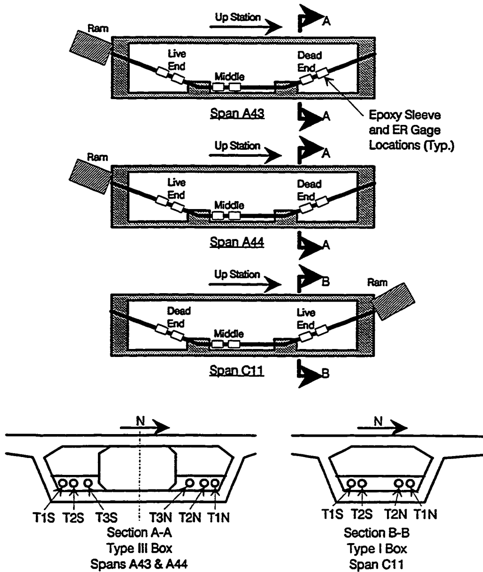
Figure 4.8 Instrumentation layouts and tendon designations.
