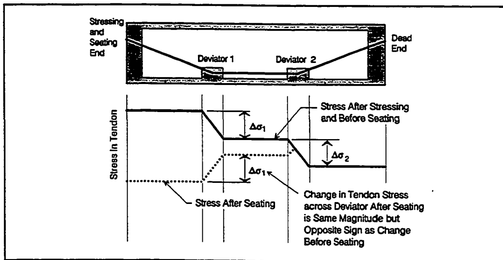
Figure 4.7 Change in tendon stress due to movement of strand during seating.
