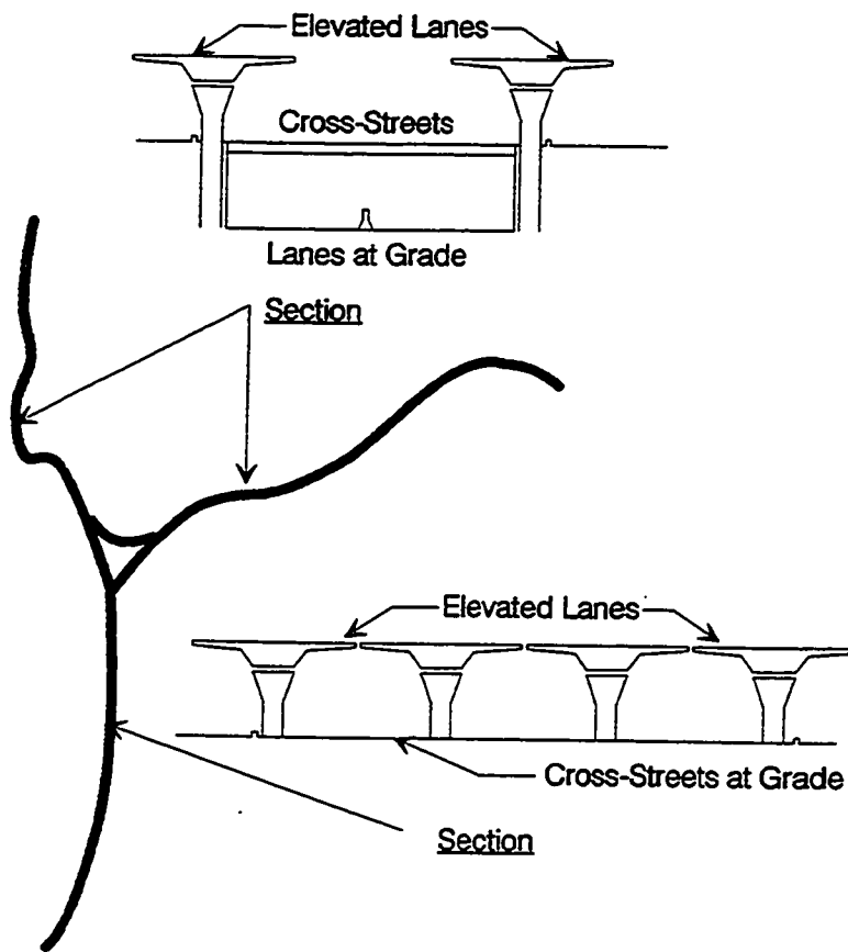
Figure 2.2 Cross-sections of the San Antonio "Y" Project.
