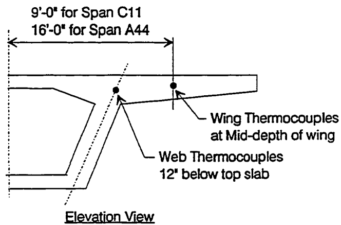
Figure 3.22 c) Typical horizontal thermocouple layout.
