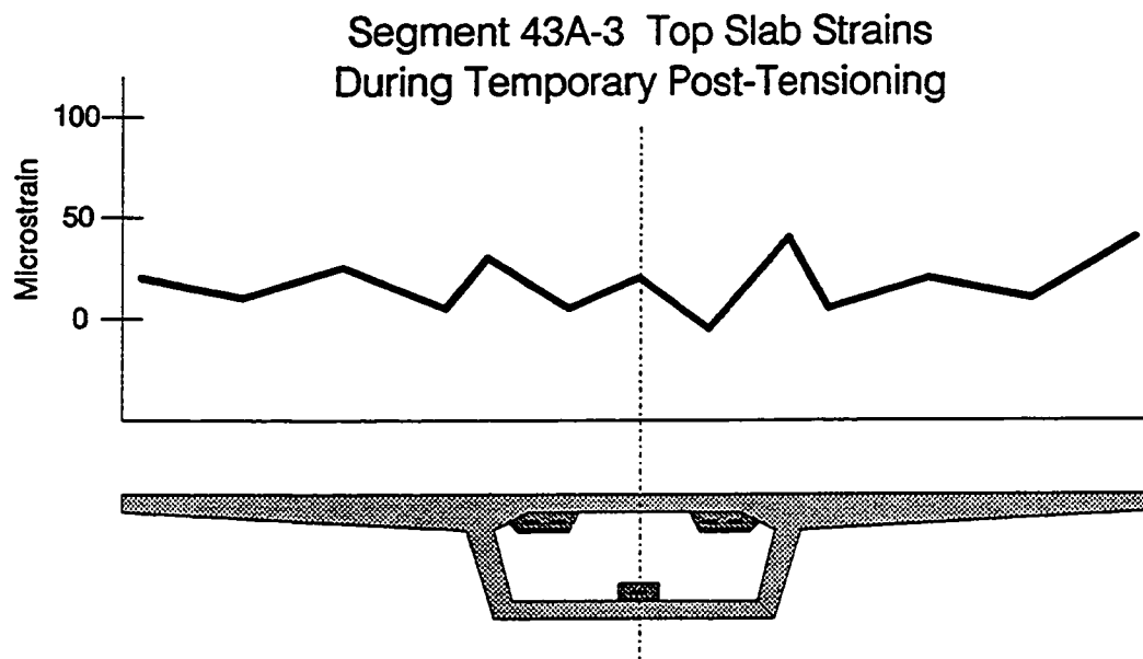
Figure 7.13 Typical uniform strain distribution across joint during temporary post-tensioning.
