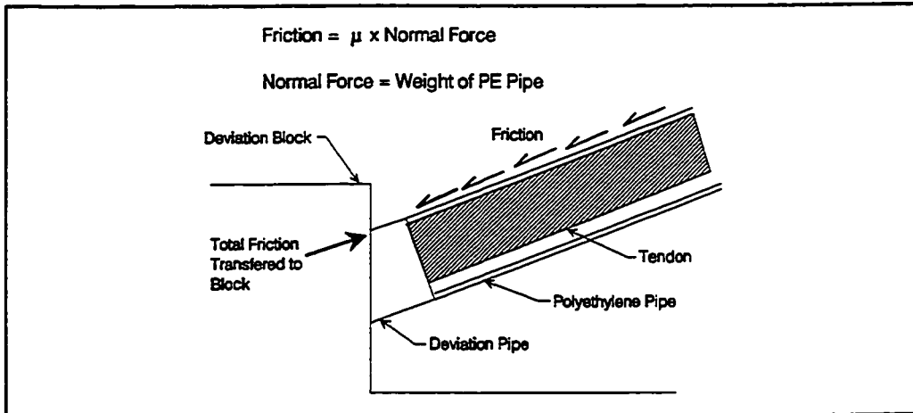
Figure 4.5 Wobble in external tendons.
