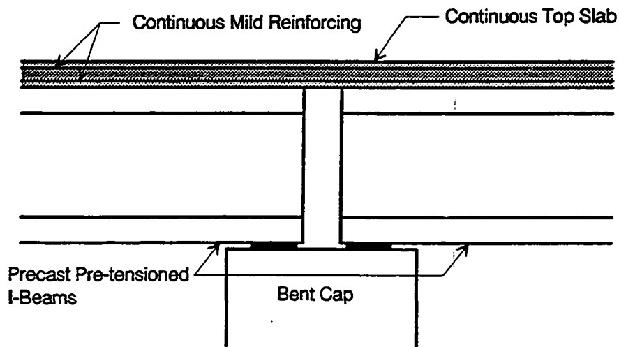
Figure 10.2 "Poor-boy" continuity between precast I-beams.
