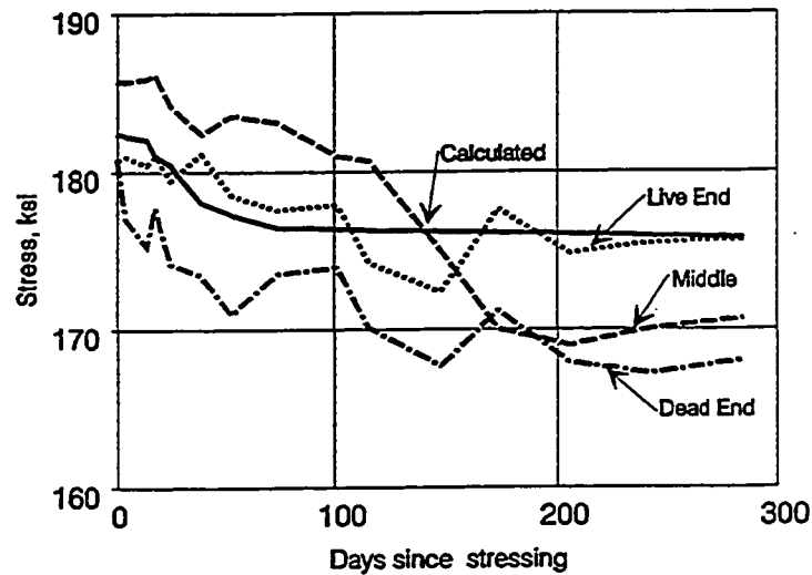
Long Term Prestress Losses Span A44 - Tendon T1S
