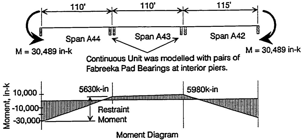
Figure 6.24 Determination of restraint moments for July 16, 1992.
