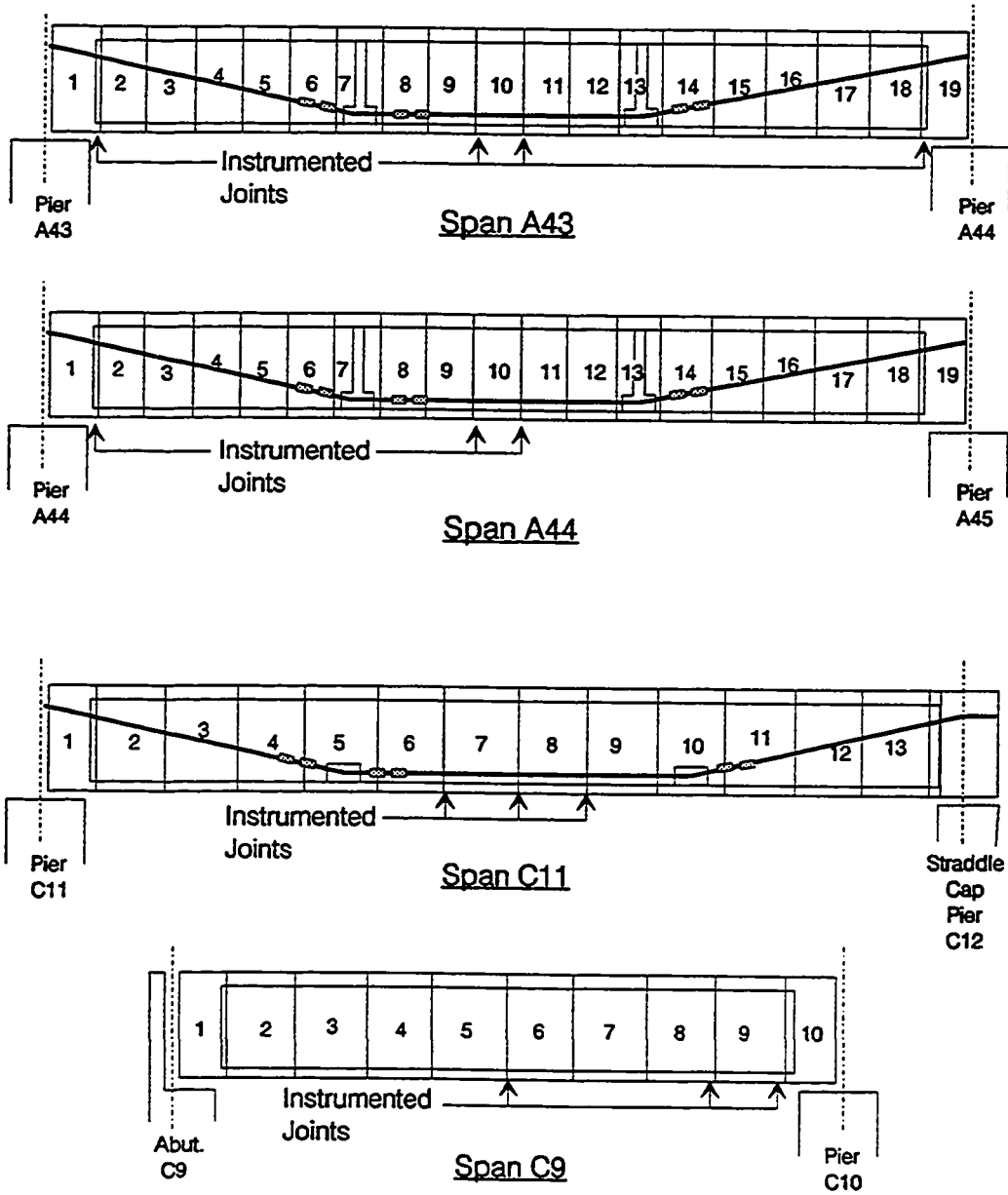
Figure 3.25 b) Joint movement instrumentation layouts.
