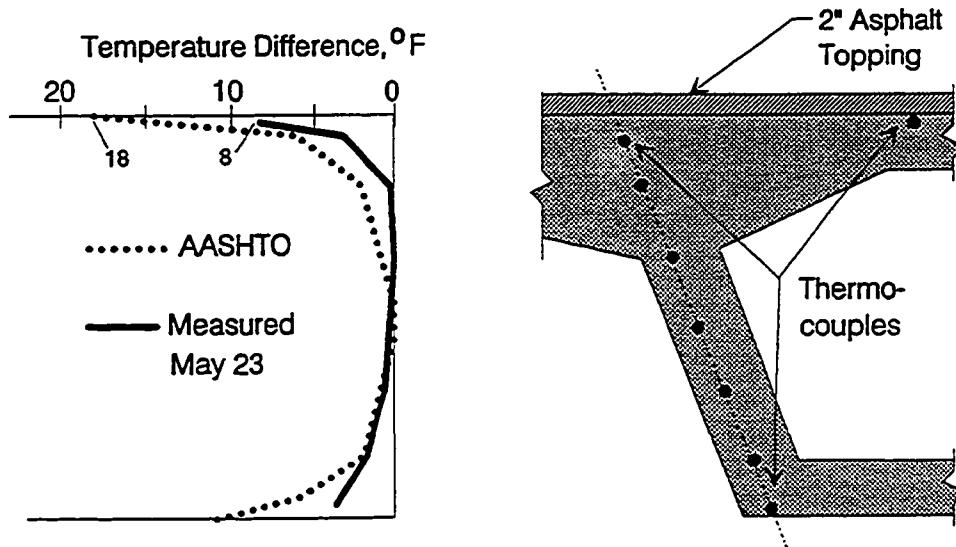
Figure 6.20 b) Maximum negative temperature gradient recorded between March 26, 1993 and May 25, 1993 (2 in. asphalt topping). Gradient occurred May 23, 1993.
