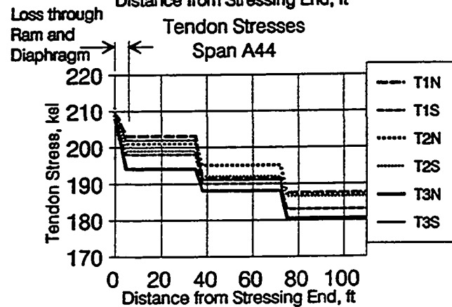
Figure 4.10 Tendon stresses after stressing, before seating.
