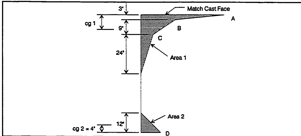
Figure 11.10 Thermal gradient in match cast segment.
