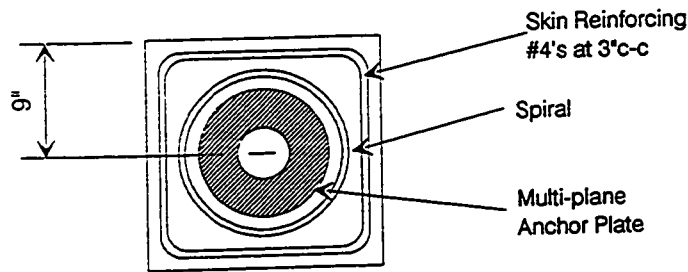
Anchorage Device and Reinforcing in Local Zone Test Specimen
