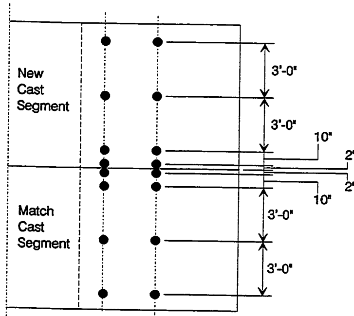
Top View of Segments
