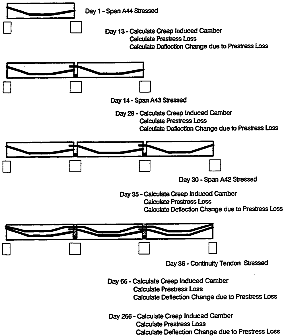
Figure 4.21 a) Erection schedule and operations of long term analysis for Spans A43 and A44.
