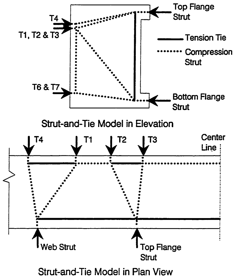
Figure 8.8 Two dimensional strut-and-tie models
