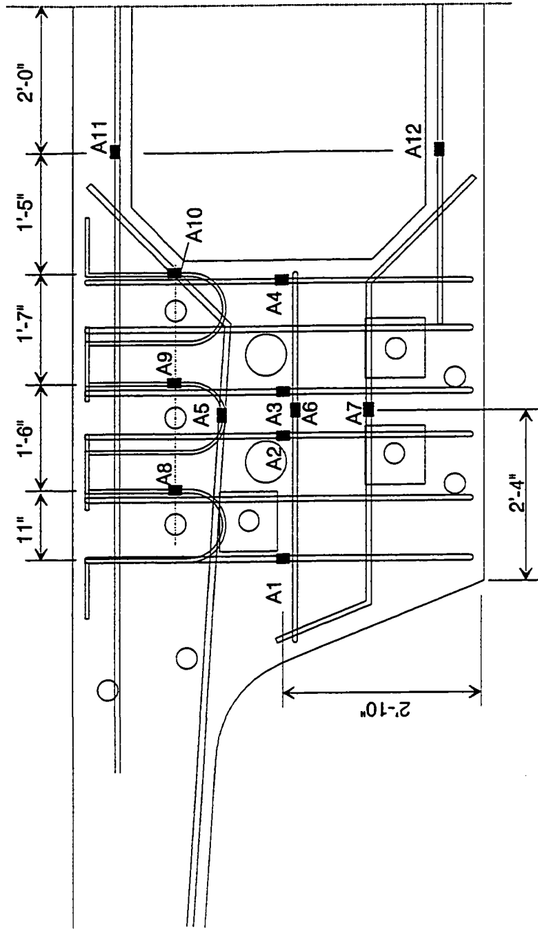
Segments 43A-1 and 44A-1 Strain Gage Layout
