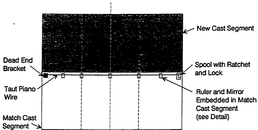
Top View of New and Match Cast Segments
