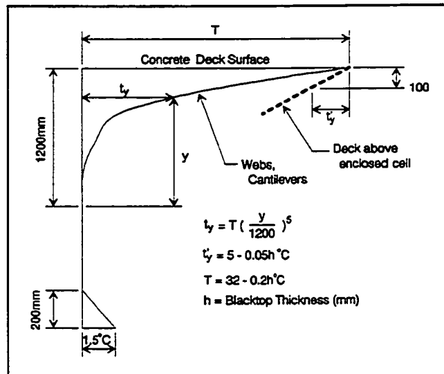
Figure 6.10 New Zealand design thermal gradient.
