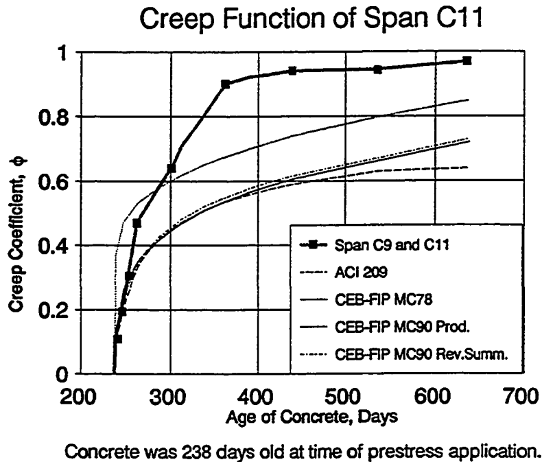
Figure 4.20 Creep functions for Spans A43, A44 and C11.
