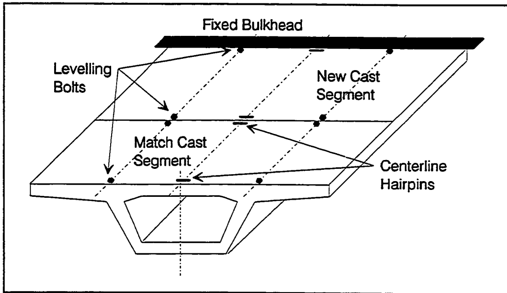
Figure 2.7 Geometry control hairpins and levelling bolts.
