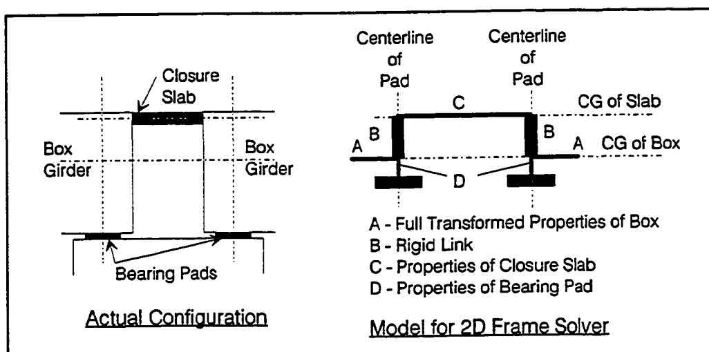
Figure 12.4 Model for "poor-boy" closure slab area.
