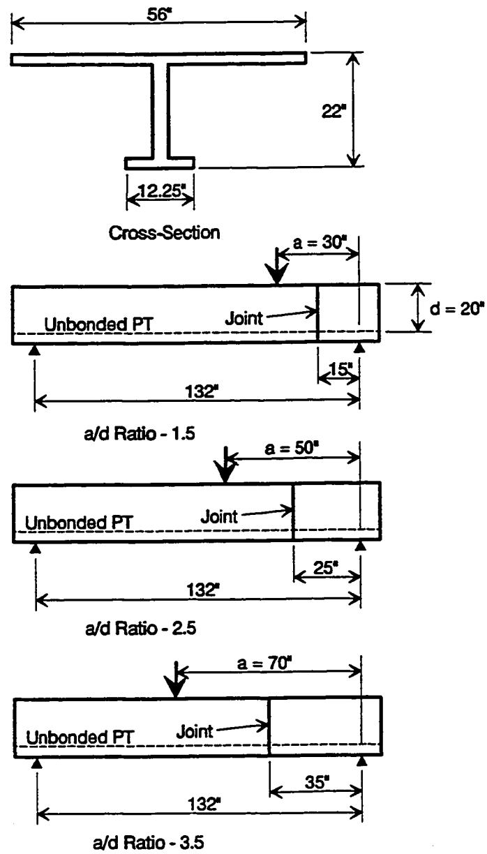
Figure 7.6 Specimens by Ramirez.
