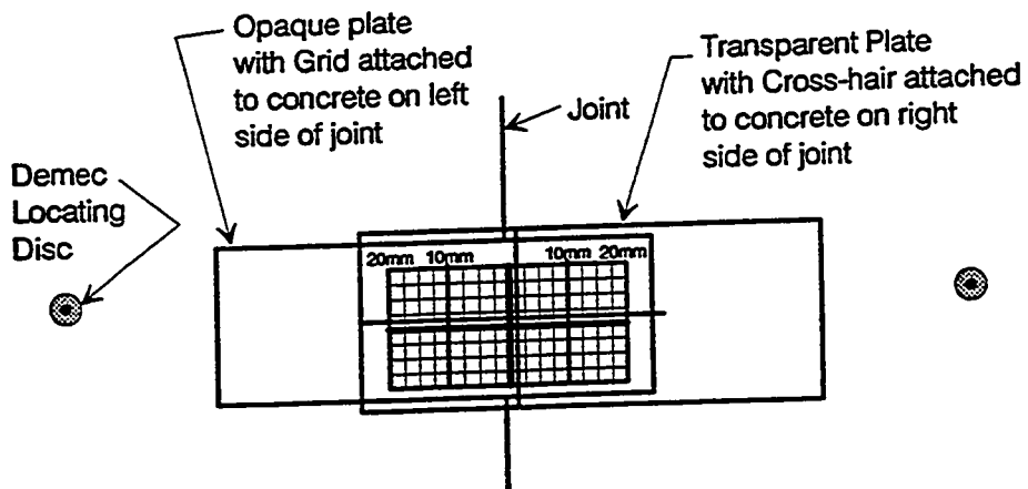
Figure 3.23 Grid crack monitor and demec points.
