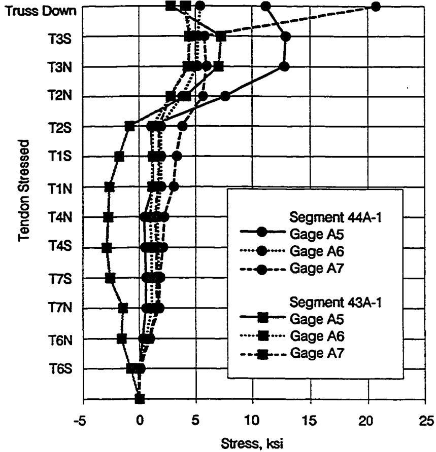
Figure 8.13 Stresses in horizontal reinforcing bars.
