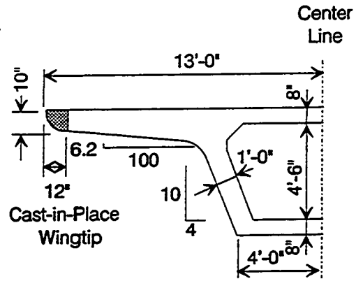
a) Typical Type I Segment Spans C9 and C11
