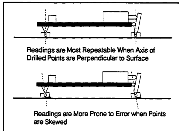
Figure 3.15 Proper and improper Demec point attachment.
