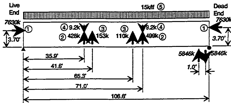
Span A43 Loading Diagram for SHLAG
