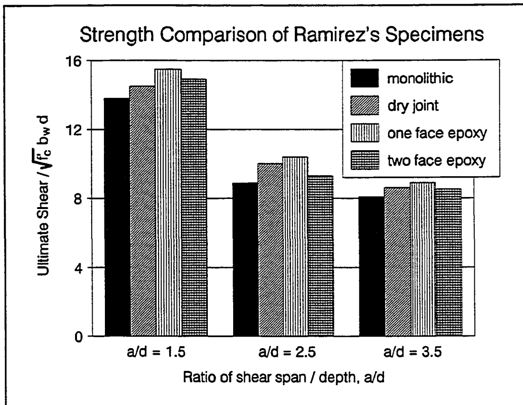
Figure 7.7 Strength comparison of Ramirez's specimens.
