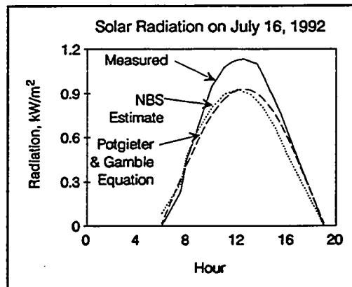
Figure 6.22 Solar radiation on July 16, 1992.
