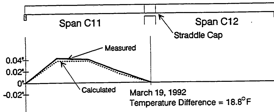
Figure 6.28 Measured and calculated deflections caused by thermal gradients in span C11.
