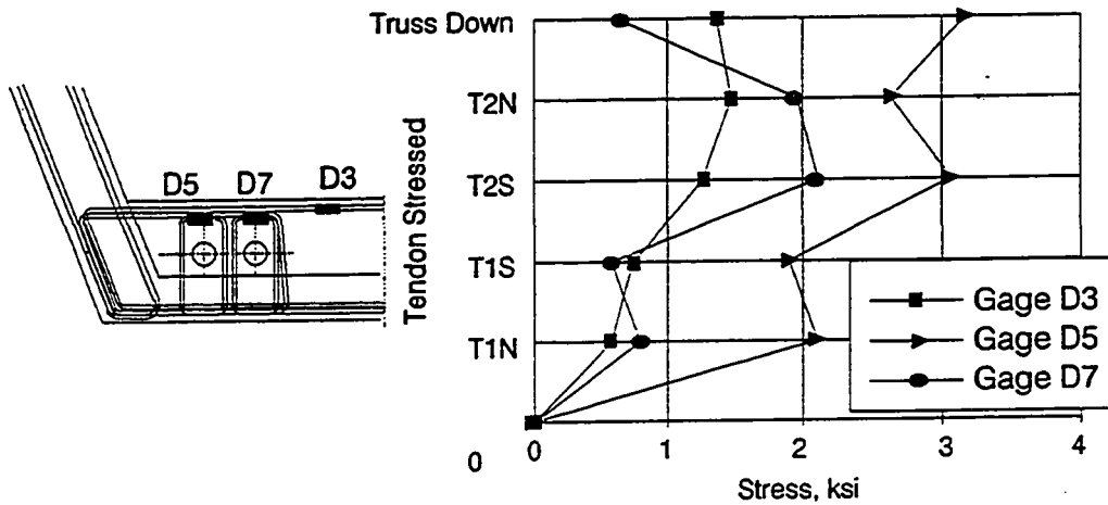
Figure 9.8 Stresses in horizontal bars.
