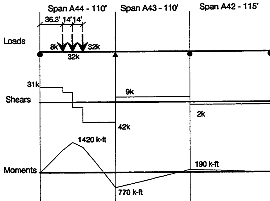
HS20-44 Truck Load
