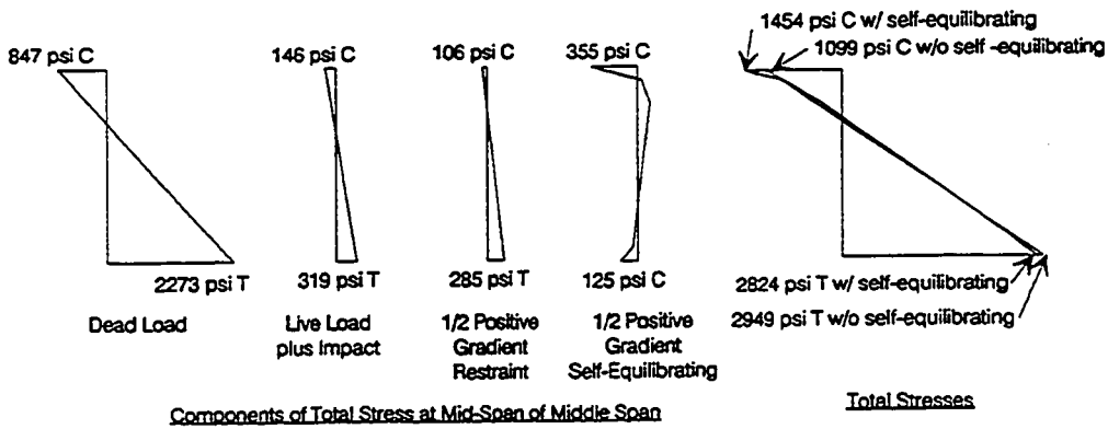
Figure 6.33 a) Comparison of bottom fiber stresses without prestressing, with and without self-equilibrating stresses.
