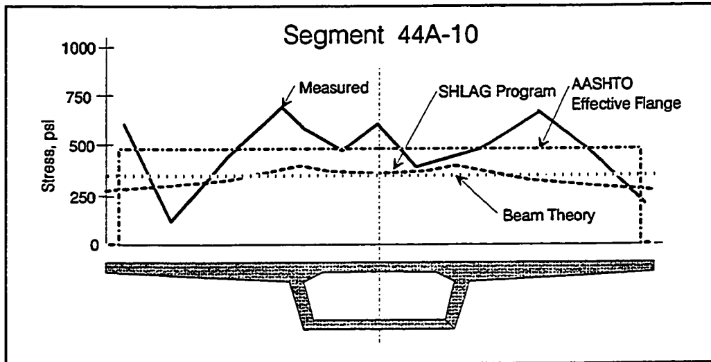
Figure 5.24 Top slab stress distribution, at mid-span, due to 54% dead load addition upon lowering erection truss.
