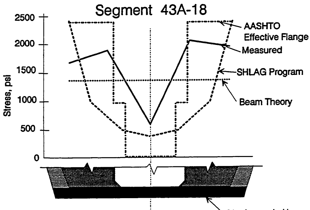
Figure 5.19 a) Bottom slab stress distributions, five feet from anchors.
