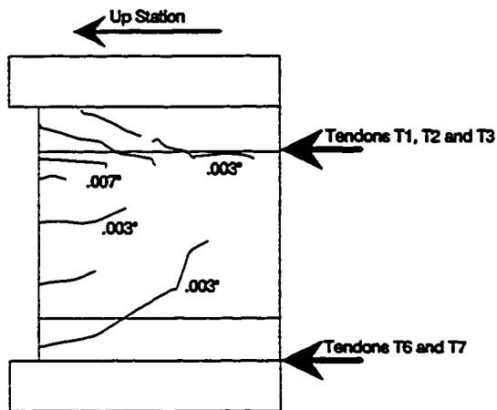
Figure 8.16 a) Segment 44A-1 north side crack patterns.
