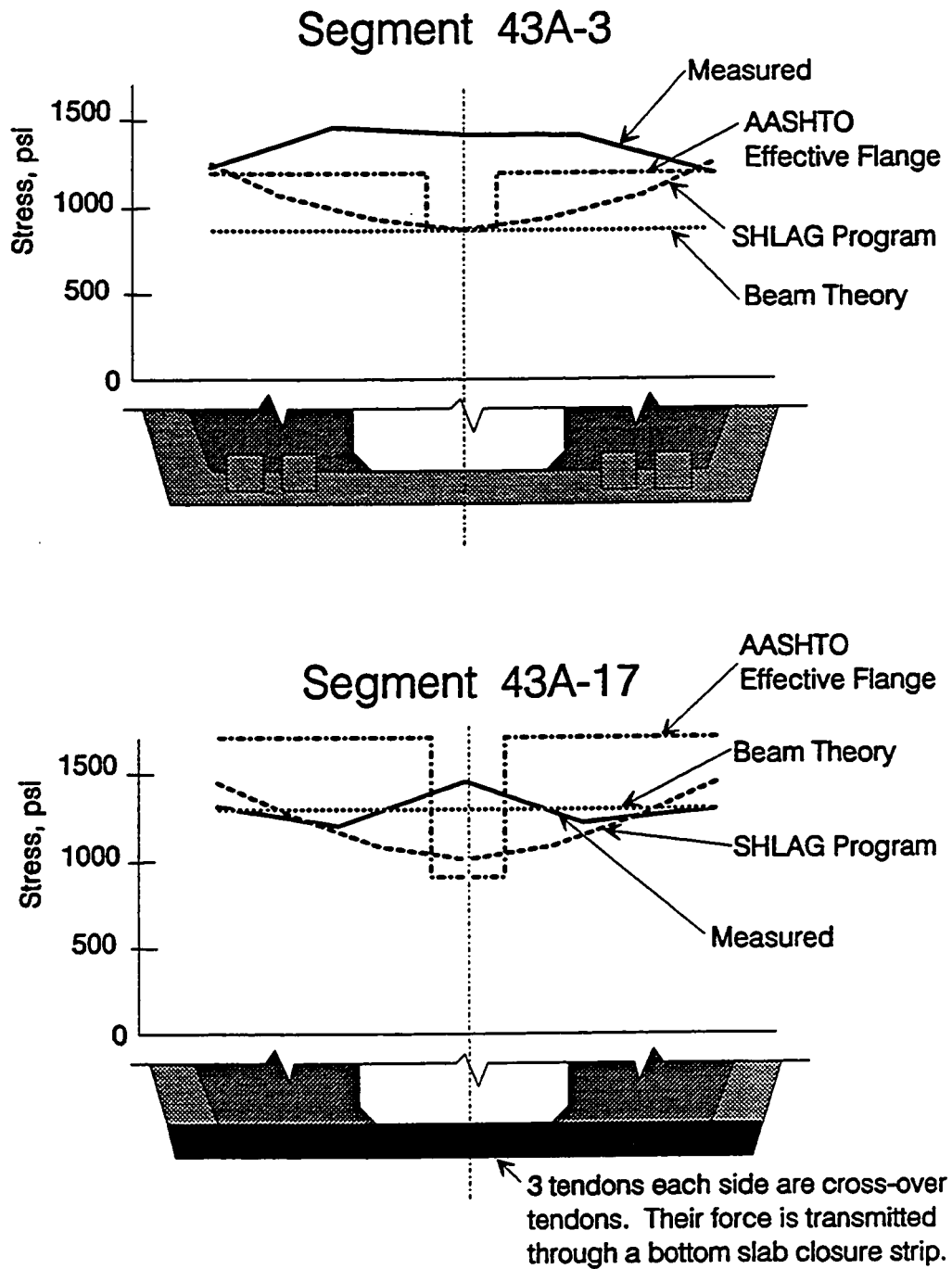
Figure 5.20 a) Bottom slab stress distributions, eleven feet from anchors.
