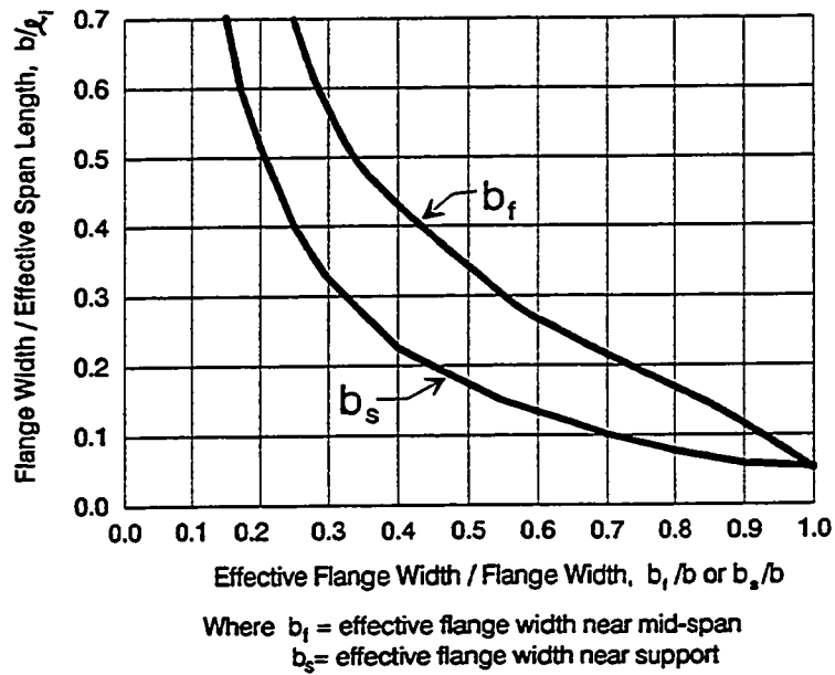
Figure 5.5 AASHTO effective flange width graph.
