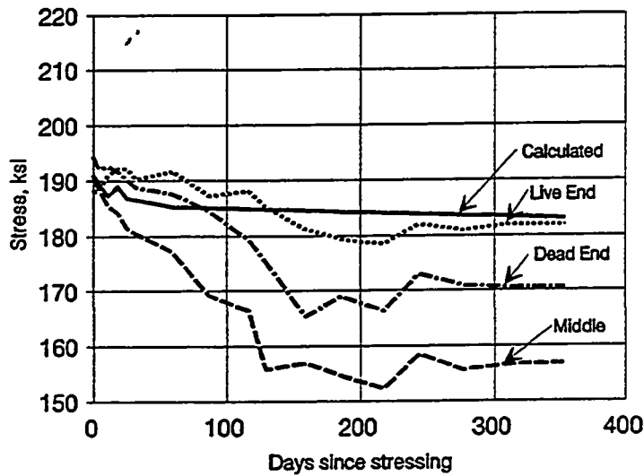
Figure 4.33 Adjusted average tendon stresses for Tendons T2N and T2S in Span C11.
