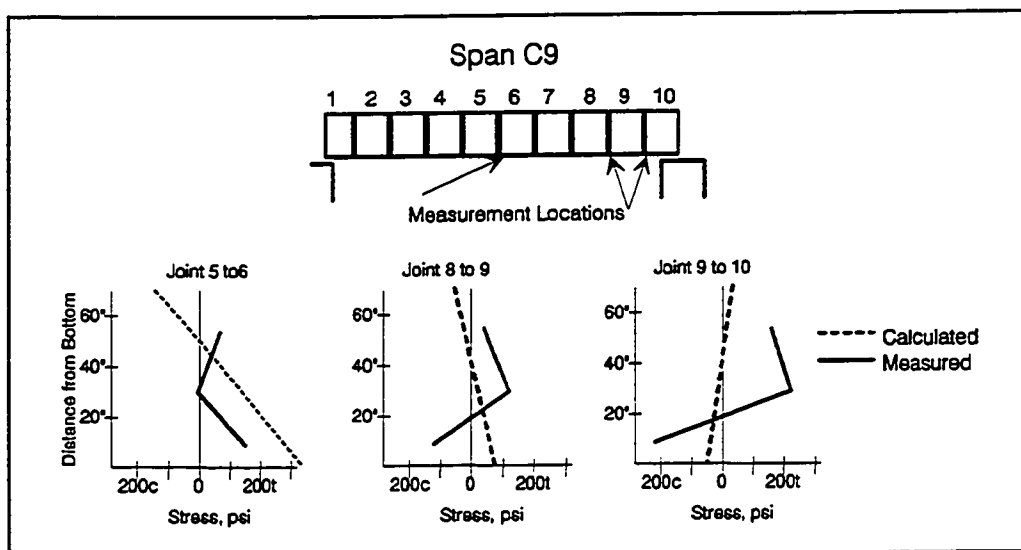
Figure 10.22 Web stresses in span C9 with live load on C9.
