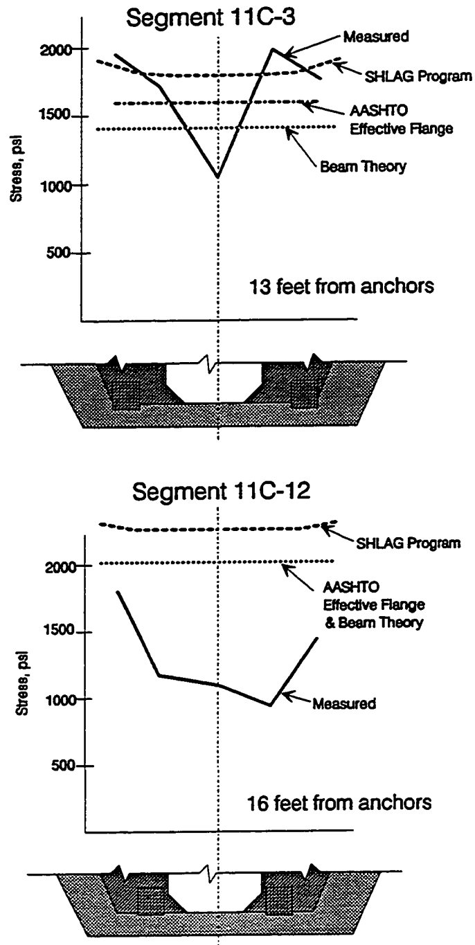
Figure 5.20 c) Bottom slab stress distributions, two segments from anchors.
