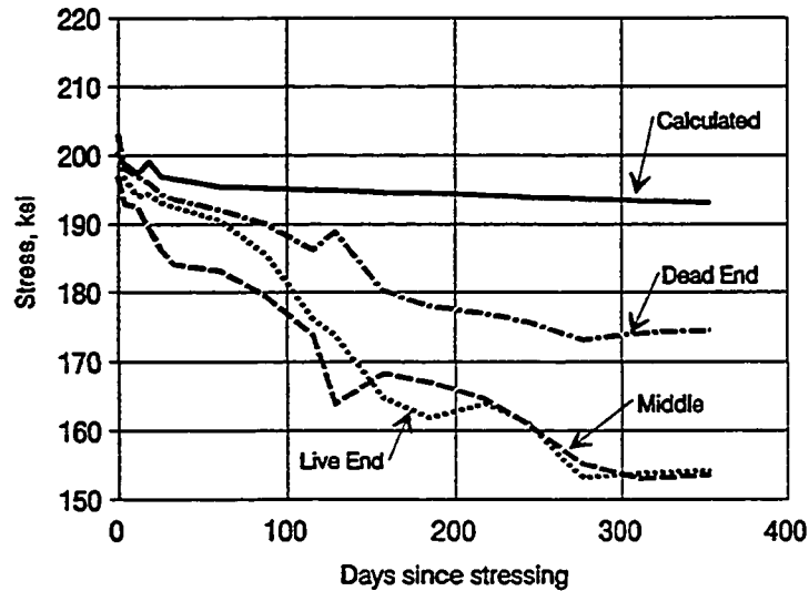
Figure 4.32 Adjusted average tendon stresses for Tendons T1N and T1S in Span C11.
