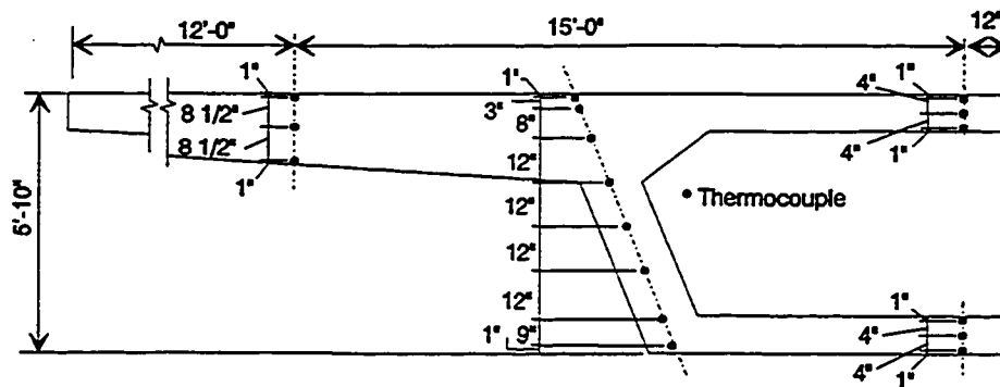
Segments 44A-6 and 44A-15 Vertical Thermocouple Layout
