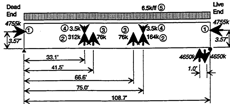
Span C11 Loading Diagram for SHLAG
