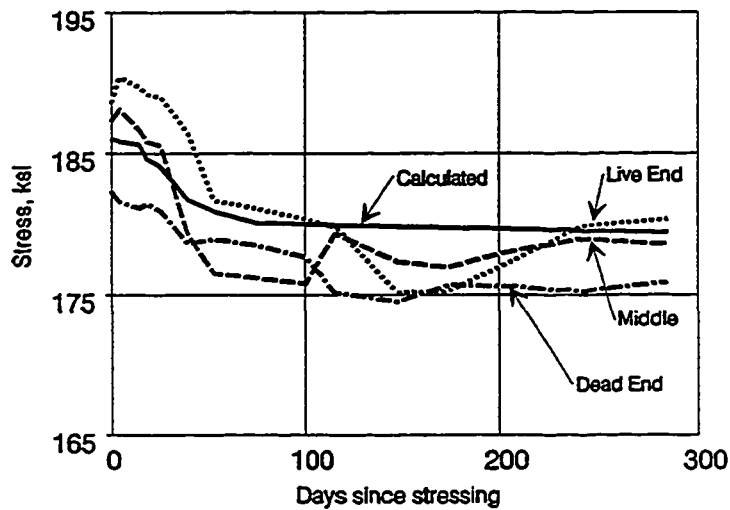
Figure 4.31 Adjusted average tendon stresses for Tendons T3N and T3S in Span A44.
