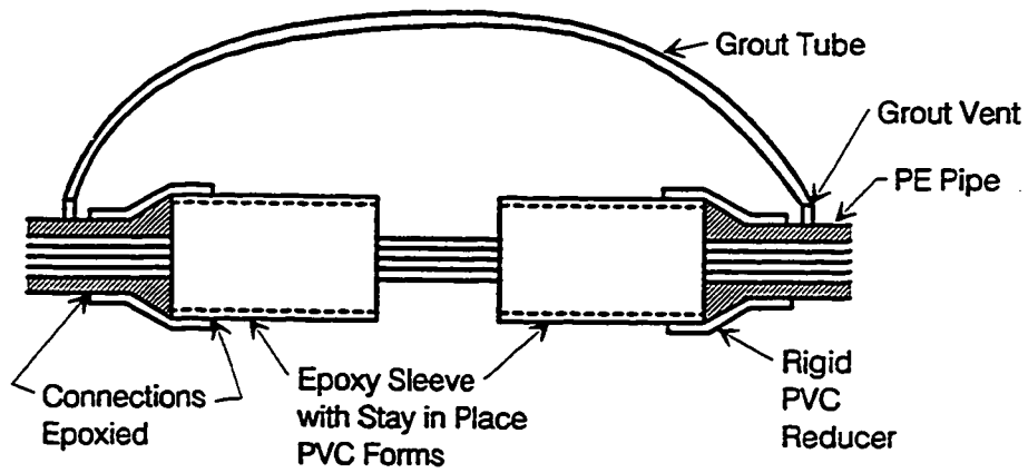
Figure 3.10 b) Grout by-pass system for Spans A43 and A44.
