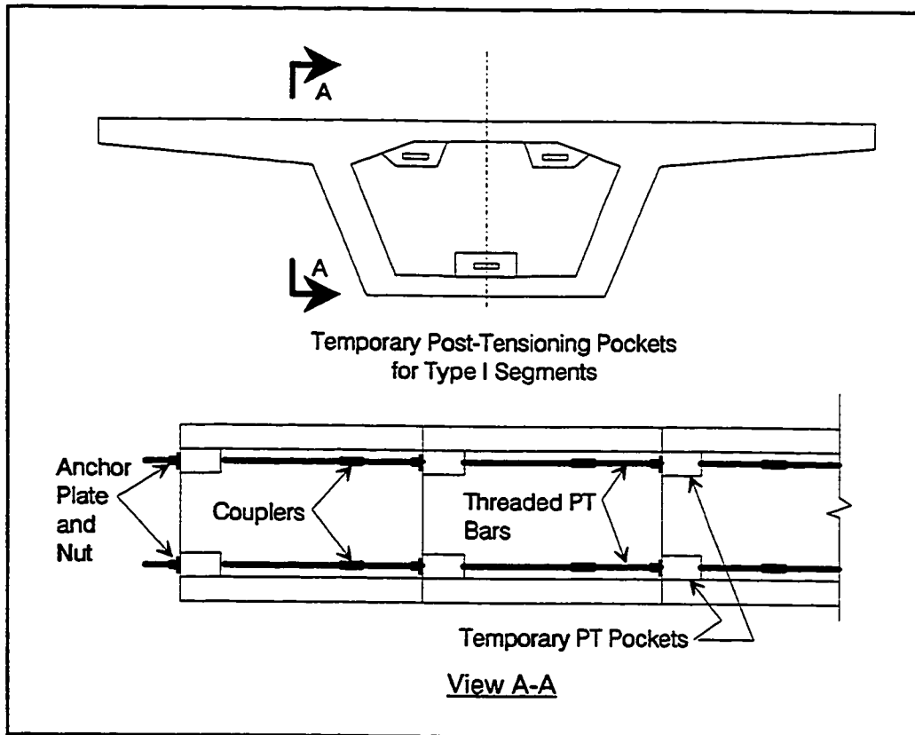
Figure 2.8 Temporary post-tensioning pockets.
