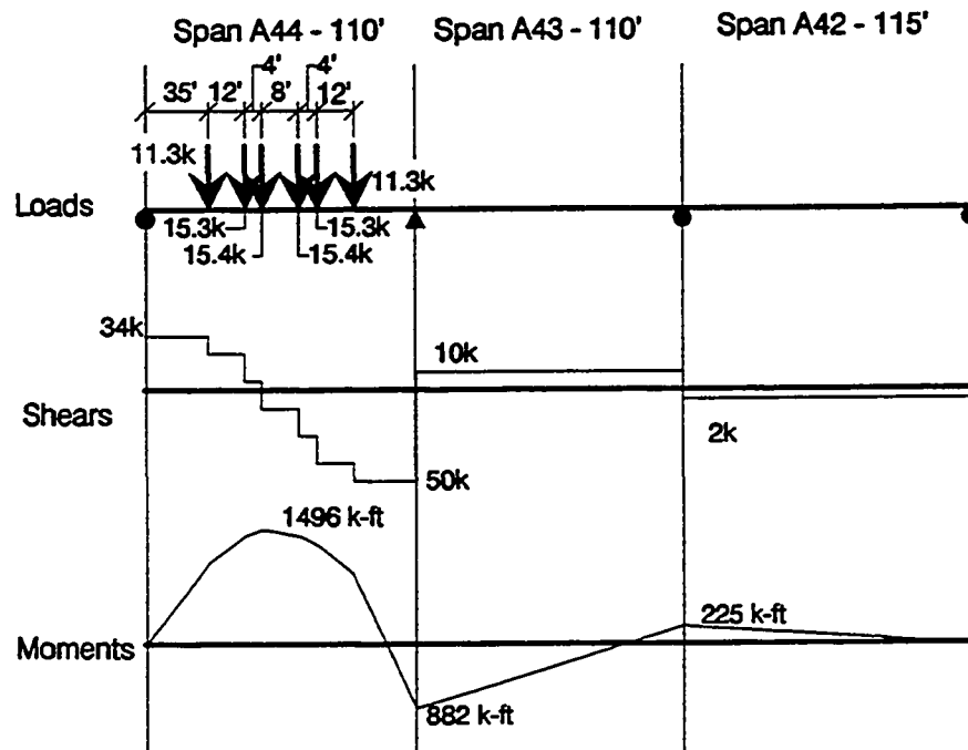
Two Dump Truck Loads
