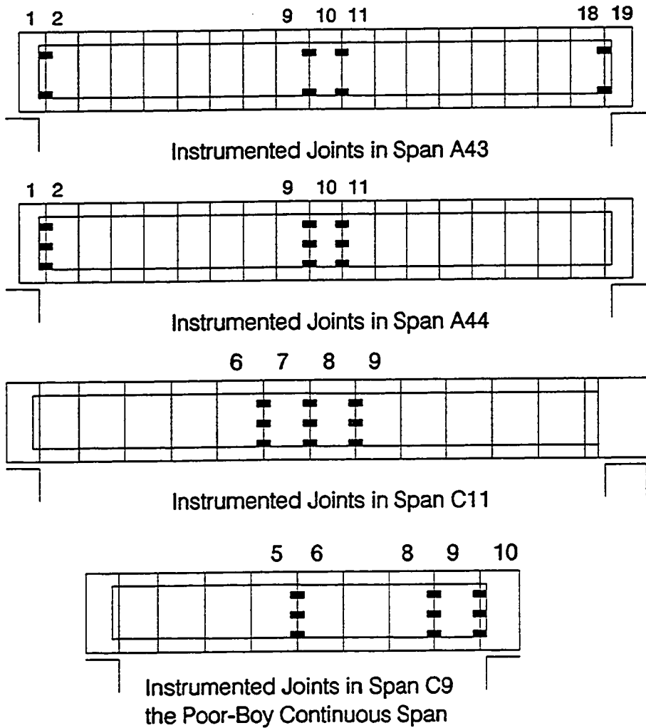
Figure 7.10 Instrumentation layouts.
