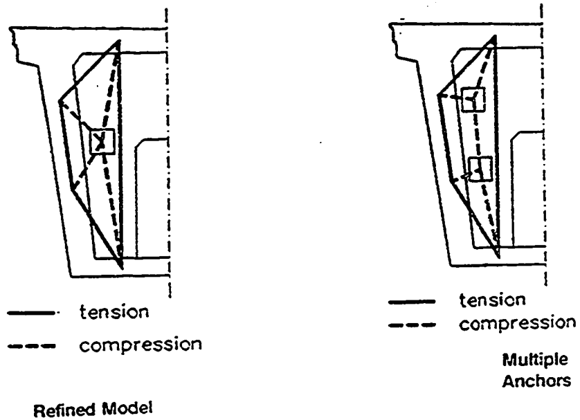
Figure 8.18 Strut-and-tie model developed by Wollmann for laboratory specimens.
