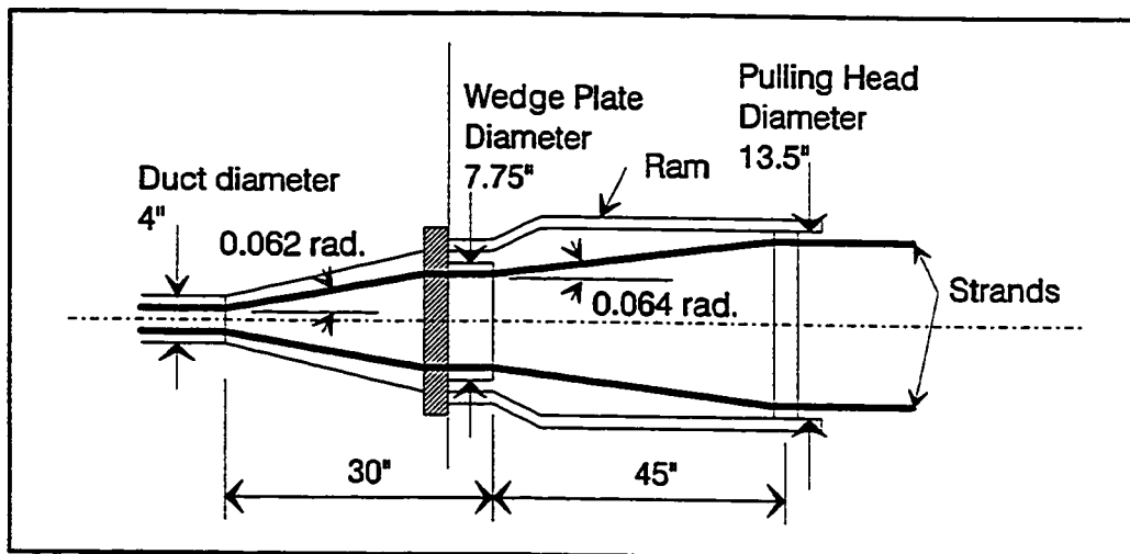
Figure 4.1 Angle changes in strands passing from duct through anchorage device and ram.
