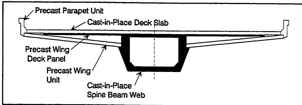
Figure 2.4 TYLI design for San Antonio "Y" Project.
