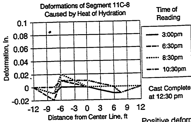
Figure 11.8 Deformed shapes.
