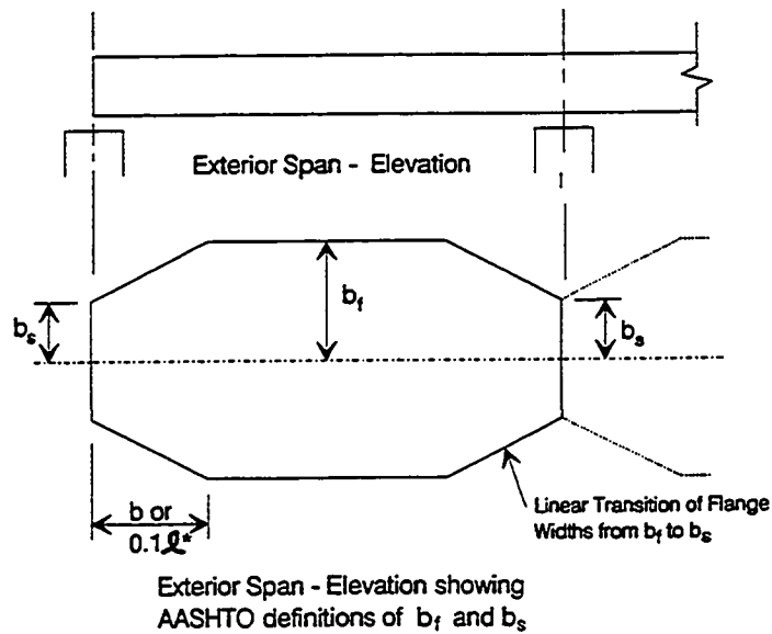
Figure 5.5 AASHTO effective flange width graph.
