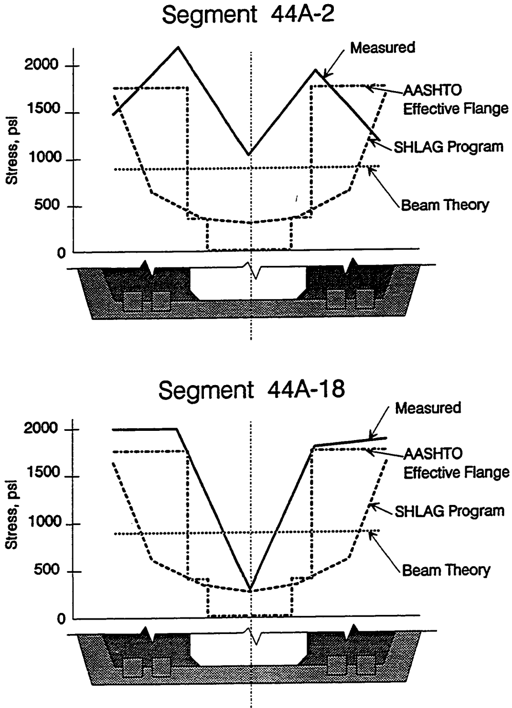
Figure 5.19 b) Bottom slab stress distributions, five feet from anchors.
