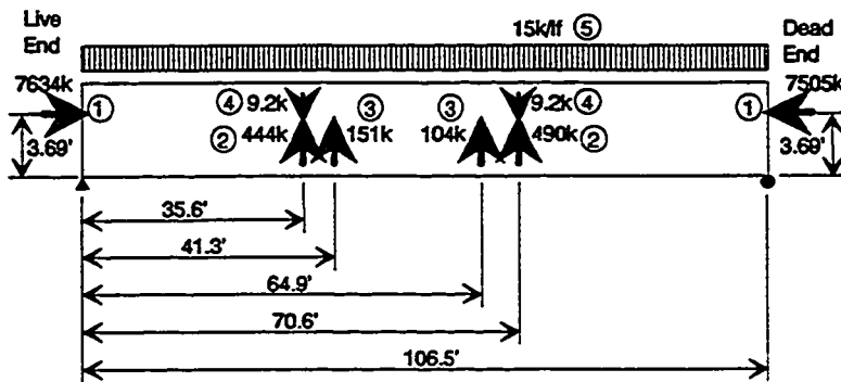
Span A44 Loading Diagram
