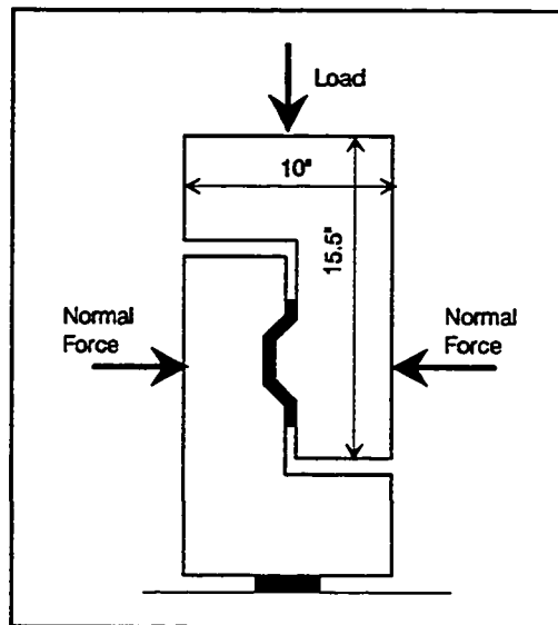
Figure 7.9 Push-off specimens by Bakhoun, Buyukozturk and Beattie.
