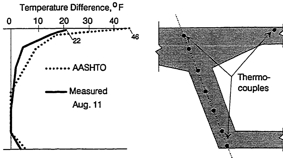
Figure 6.17 a) Maximum positive temperature gradient recorded between July 16, 1992 and March 25, 1993 (no topping). Gradient occurred August 11, 1992.
