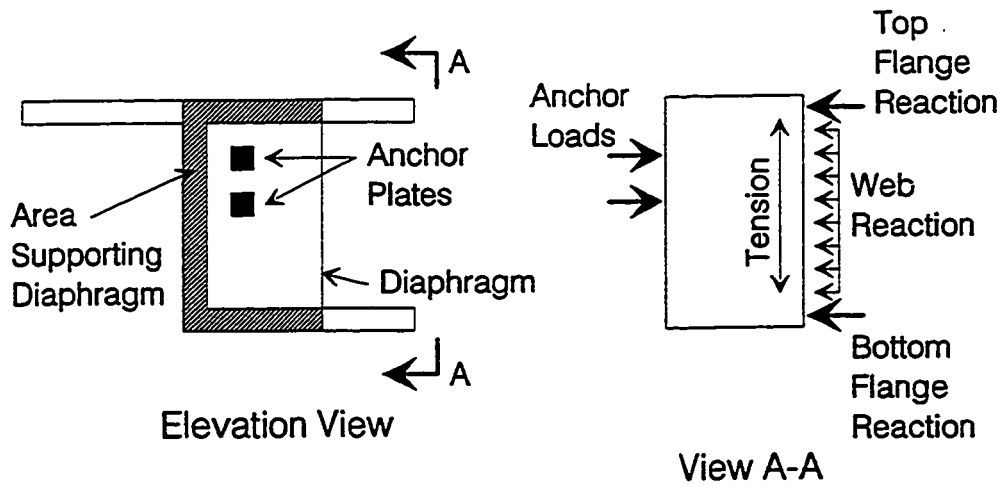
Figure 8.3 Diaphragm as deep beam supported by flanges and web.
