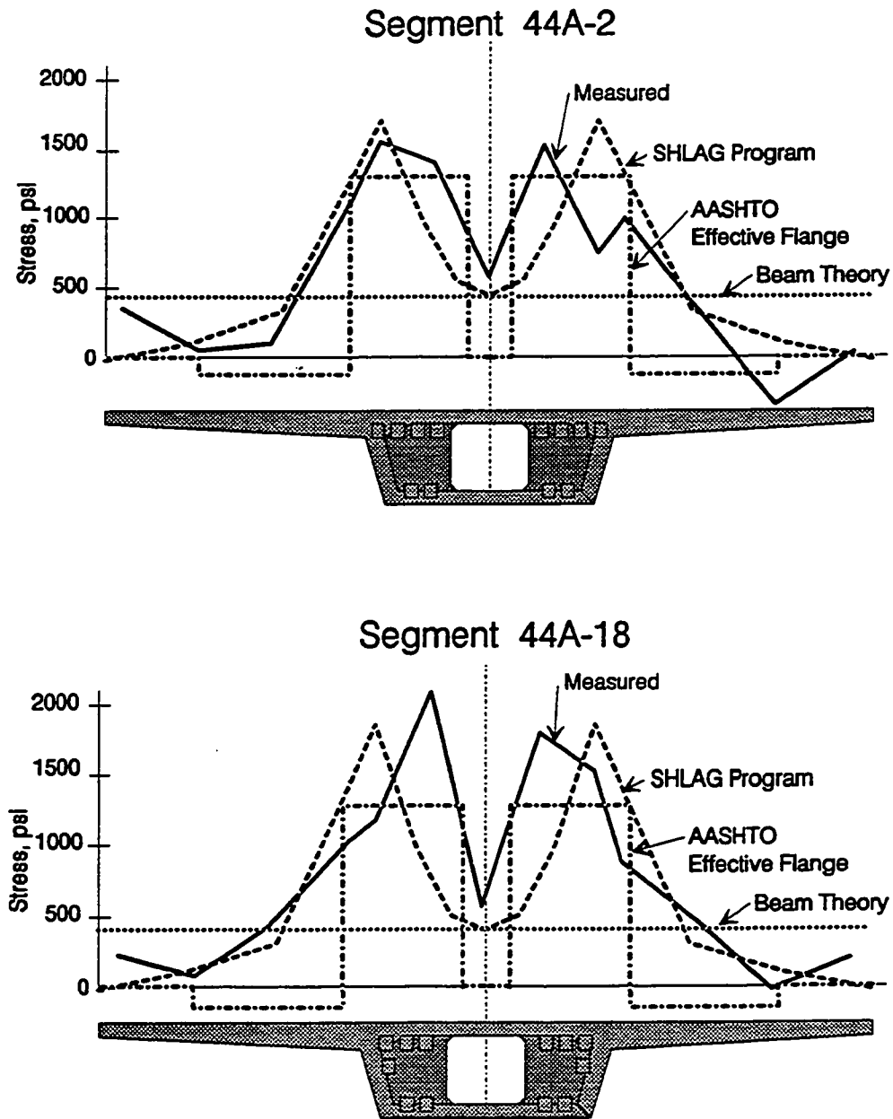
Figure 5.16 b) Top slab stress distributions, five feet from anchors.
