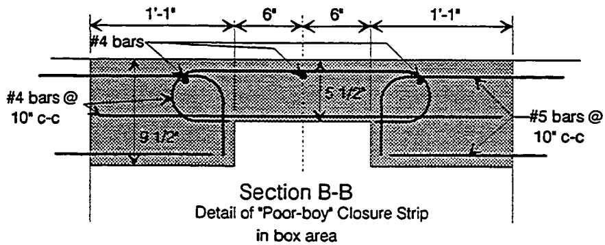
Figure 10.3 Details of "poor-boy" closure slab.
