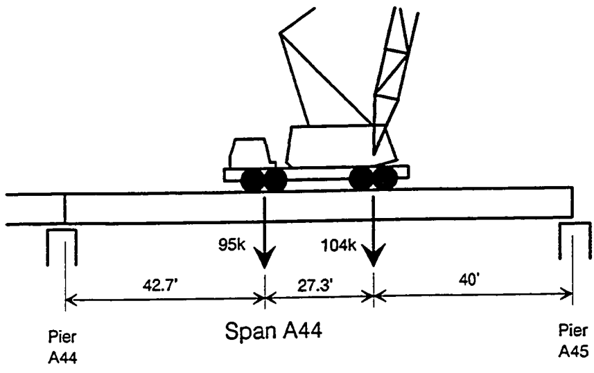
Figure 10.6 HC-238B truck crane.
