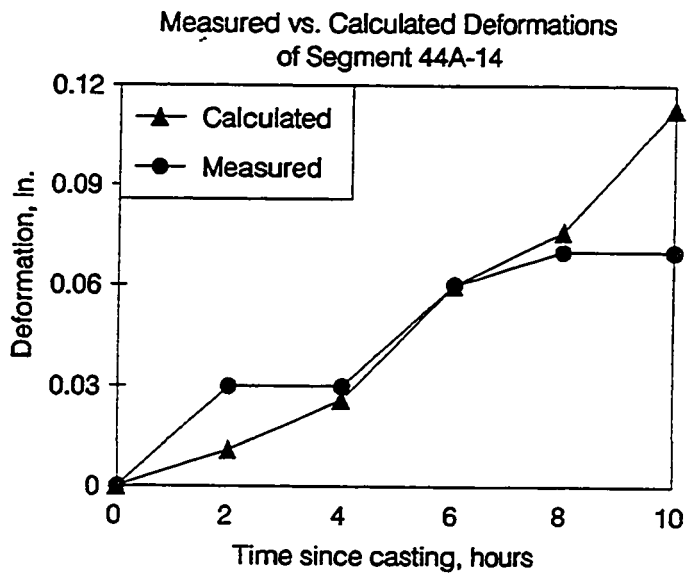
Figure 11.11 Comparison of measured and calculated deformations.
