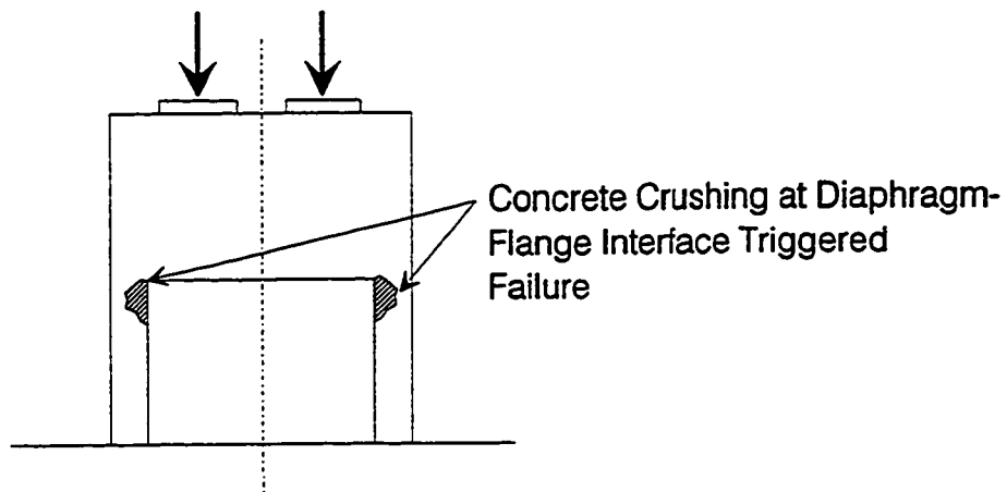
Figure 8.4 Failure of Wollmann's diaphragm specimens.
