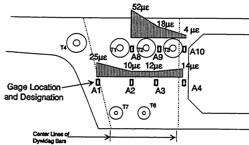
Final Strains in Vertical Reinforcing Bars After Dywidag Stressing Segment 44A-1
