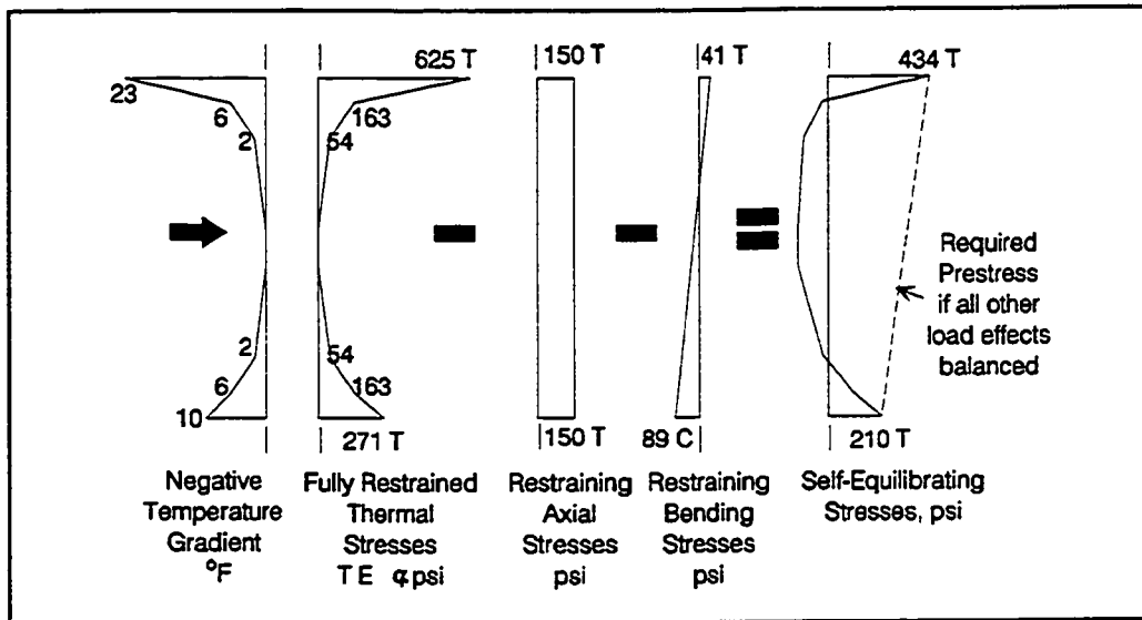
Figure 6.31 Self-equilibrating stresses for negative gradient on Type I cross-section, ignoring restraint moments.
