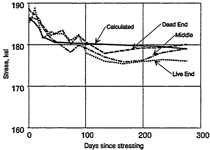
Figure 4.28 Adjusted average tendon stresses for Tendons T3N and T3S in Span A43.
