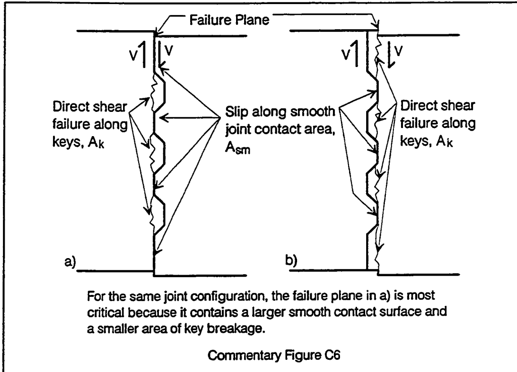
Figure 7.27 Joint shear failure plane.
