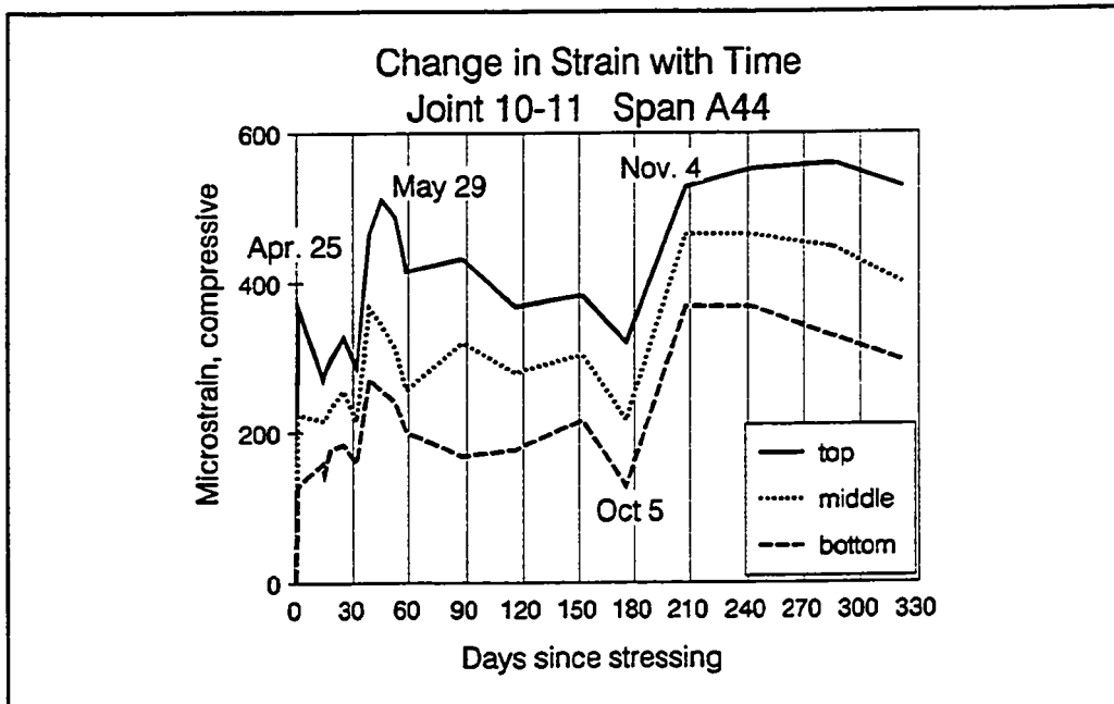
Figure 7.16 Changes in strains with time across a typical joint.
