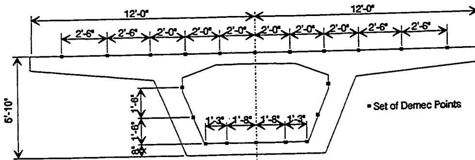
Span C11 Demec Point Layout
