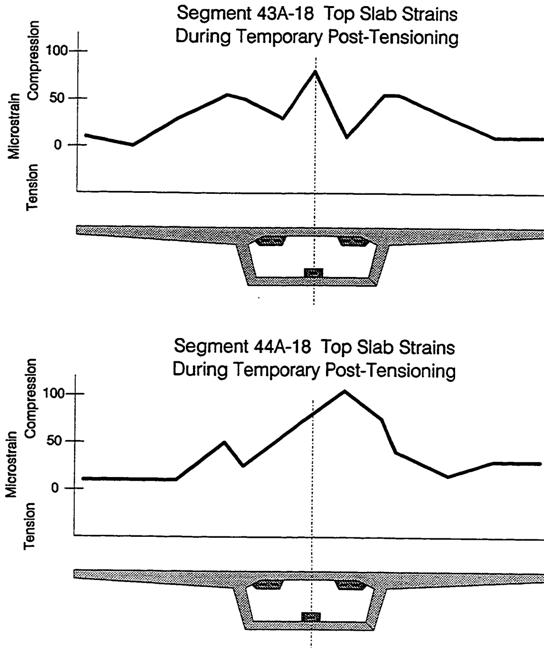
Figure 7.14 Typical non-uniform strain distributions across joints during temporary post-tensioning.
