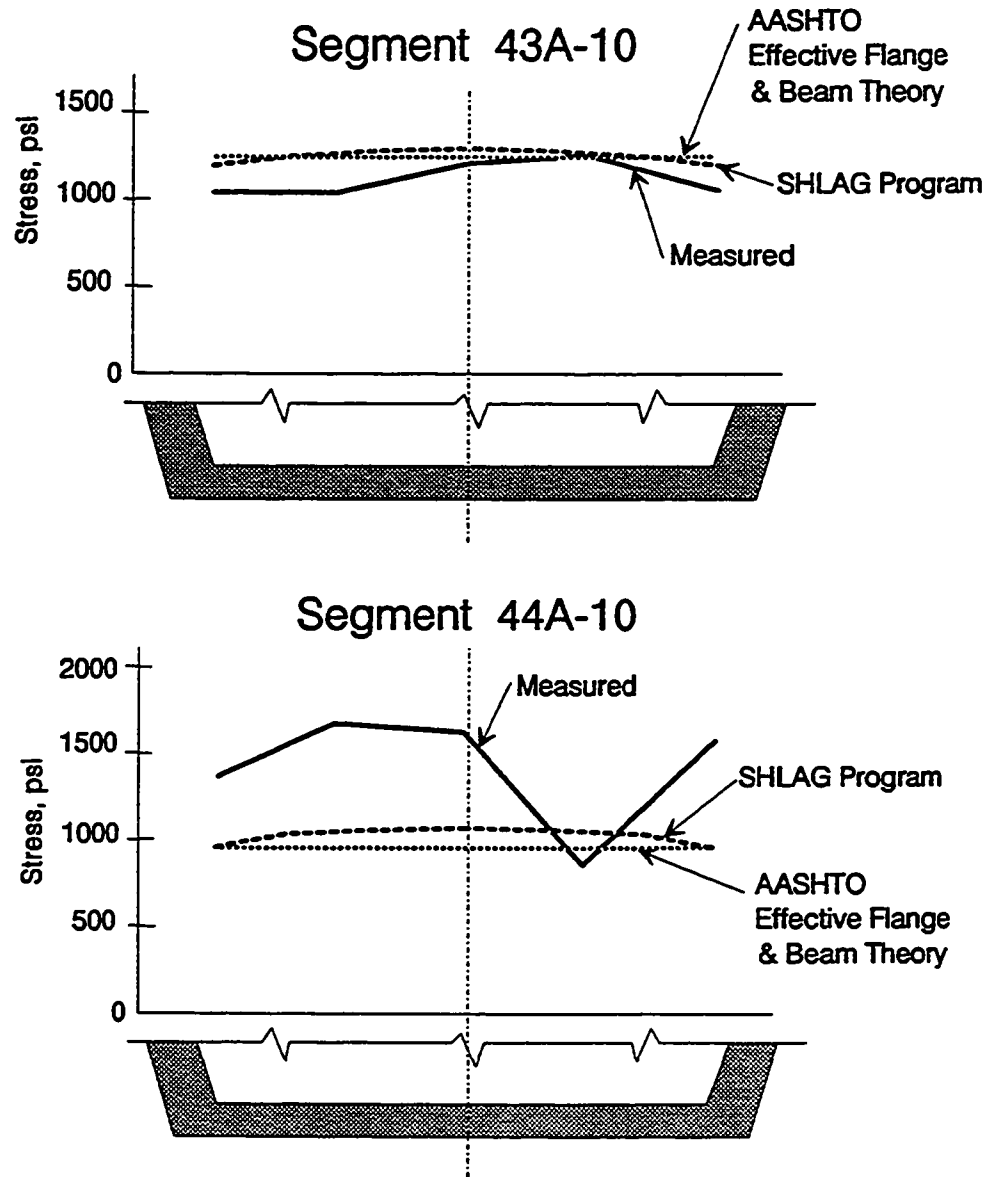
Figure 5.21 Bottom slab stress distributions, at mid-span.
