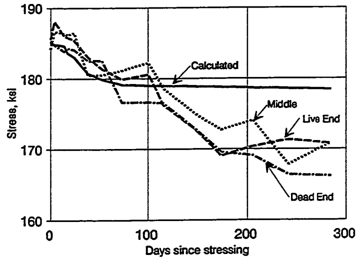
Long Term Prestress Losses Span A44 - Tendon T1N
