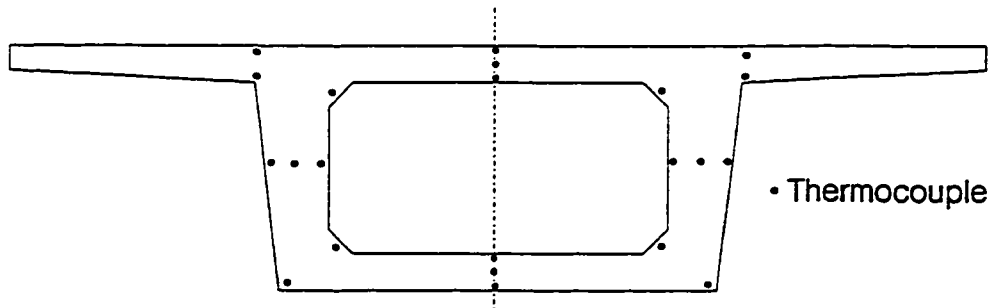
a) Thermocouple Layout for Hoffman, McClure and West Test Bridge.
