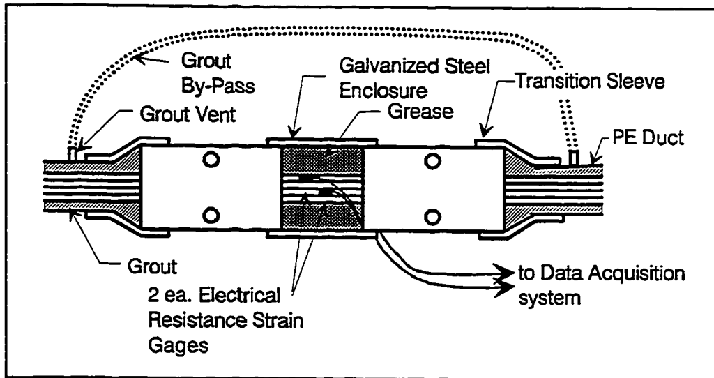
Figure 3.6 Schematic of grout by-pass system.
