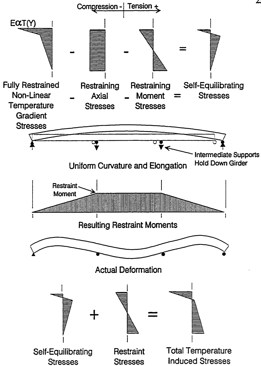
Figure 6.4 Indeterminant beam subjected to non-linear gradient.
