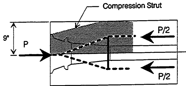
Compression Strut in Local Zone Specimen
