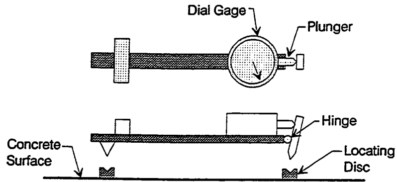
Figure 3.13 Demec extensometer.
