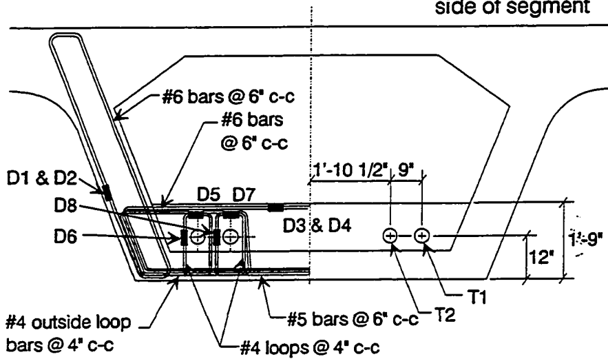
Span C11 Deviator Segment Elevation View
