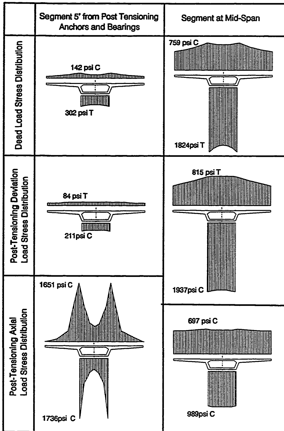
Figure 5.23 Separation of load effects.
