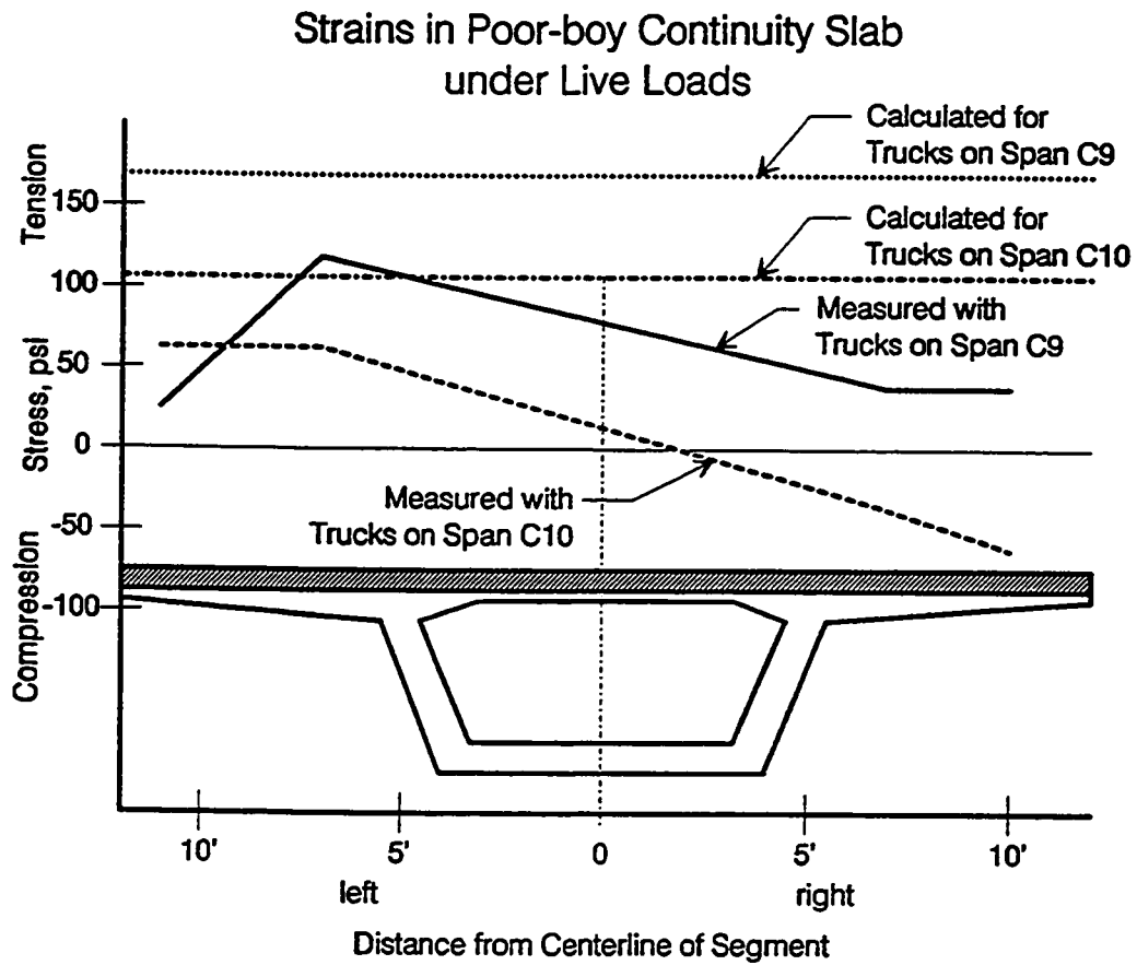
Figure 10.21 Stresses in "poor-boy" continuity slab.
