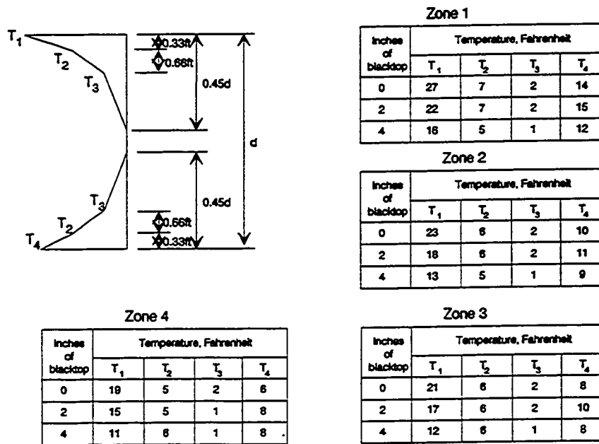
Figure 6.14 b) Design negative thermal gradients.
