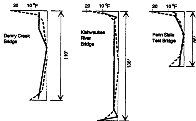
Measured Negative Gradients
