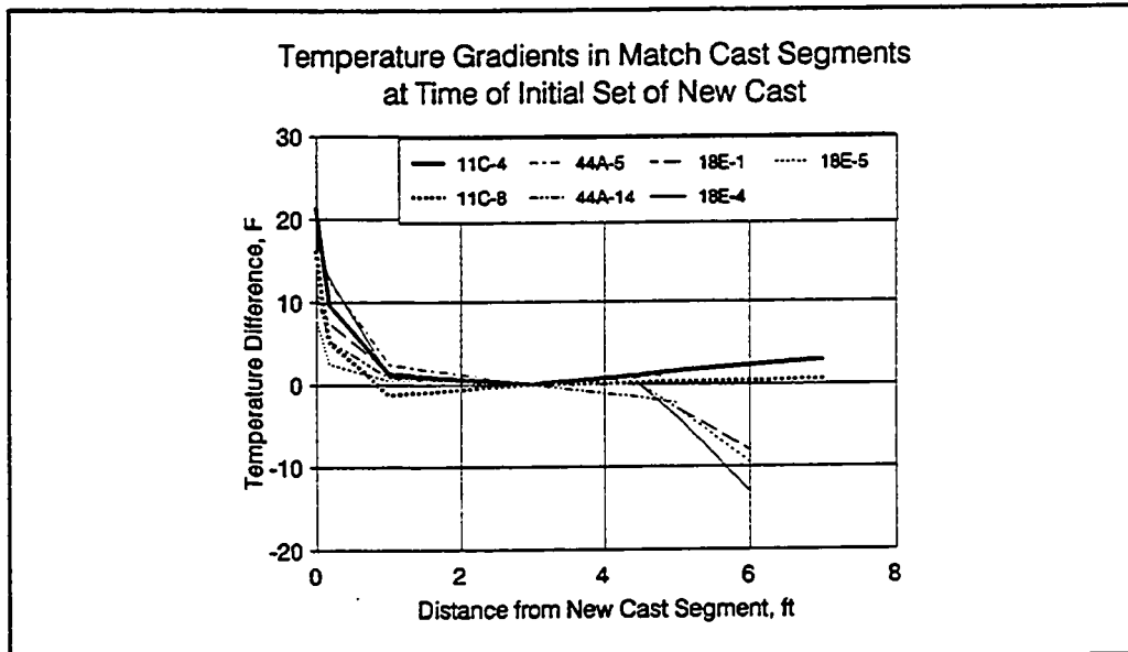
Figure 11.13 Thermal gradient in match cast segment at time of initial set of new cast segment.
