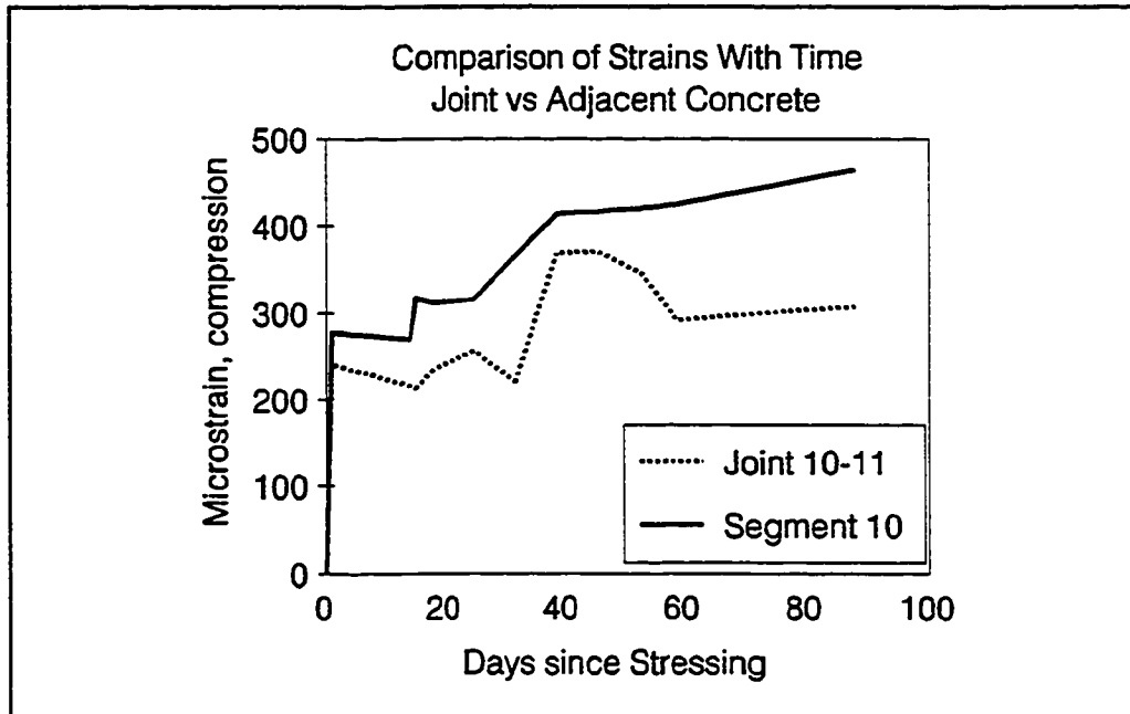
Figure 7.17 Comparison of average change in strain with time, joint vs. adjacent concrete.
