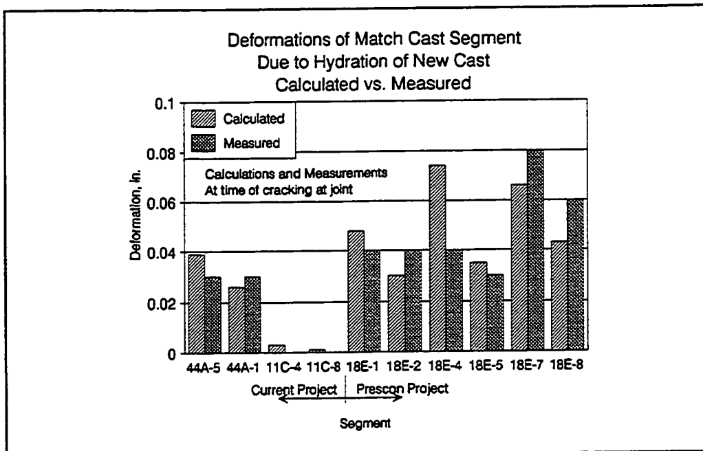
Figure 11.12 Calculated vs. measured segment deformations at time of wingtip crack opening.
