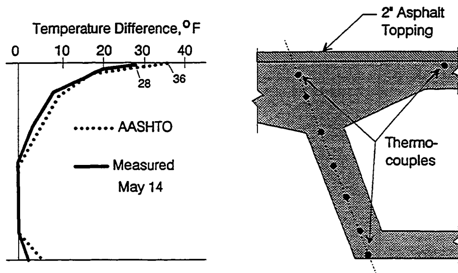
Figure 6.17 b) Maximum positive temperature gradient recorded between March 26, 1993 and May 25, 1993 (2 in. asphalt topping). Gradient occurred May 14, 1993.
