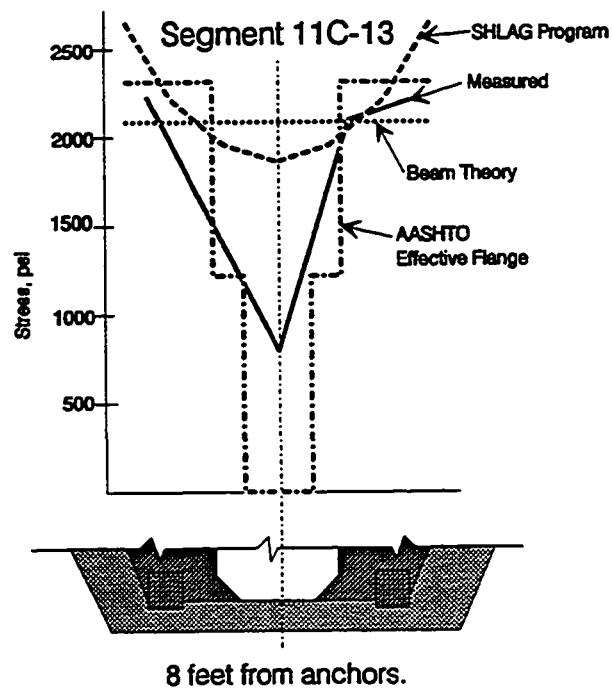
Figure 5.19 c) Bottom slab stress distributions, one segment from anchors.
