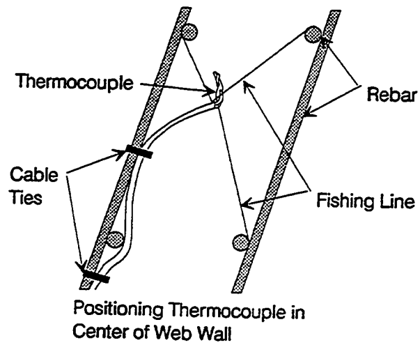
Figure 3.21 Positioning thermocouples with fishing line.
