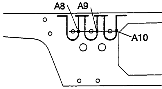
Stresses in U-Shaped Reinforcing Bars in Diaphragm Segments
