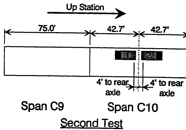
Figure 10.10 Truck positions in spans C9 and C10, "poor-boy" unit.
