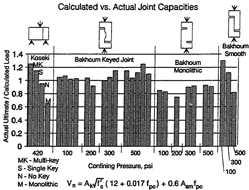
Figure 7.26 Calculated vs actual joint capacities.
