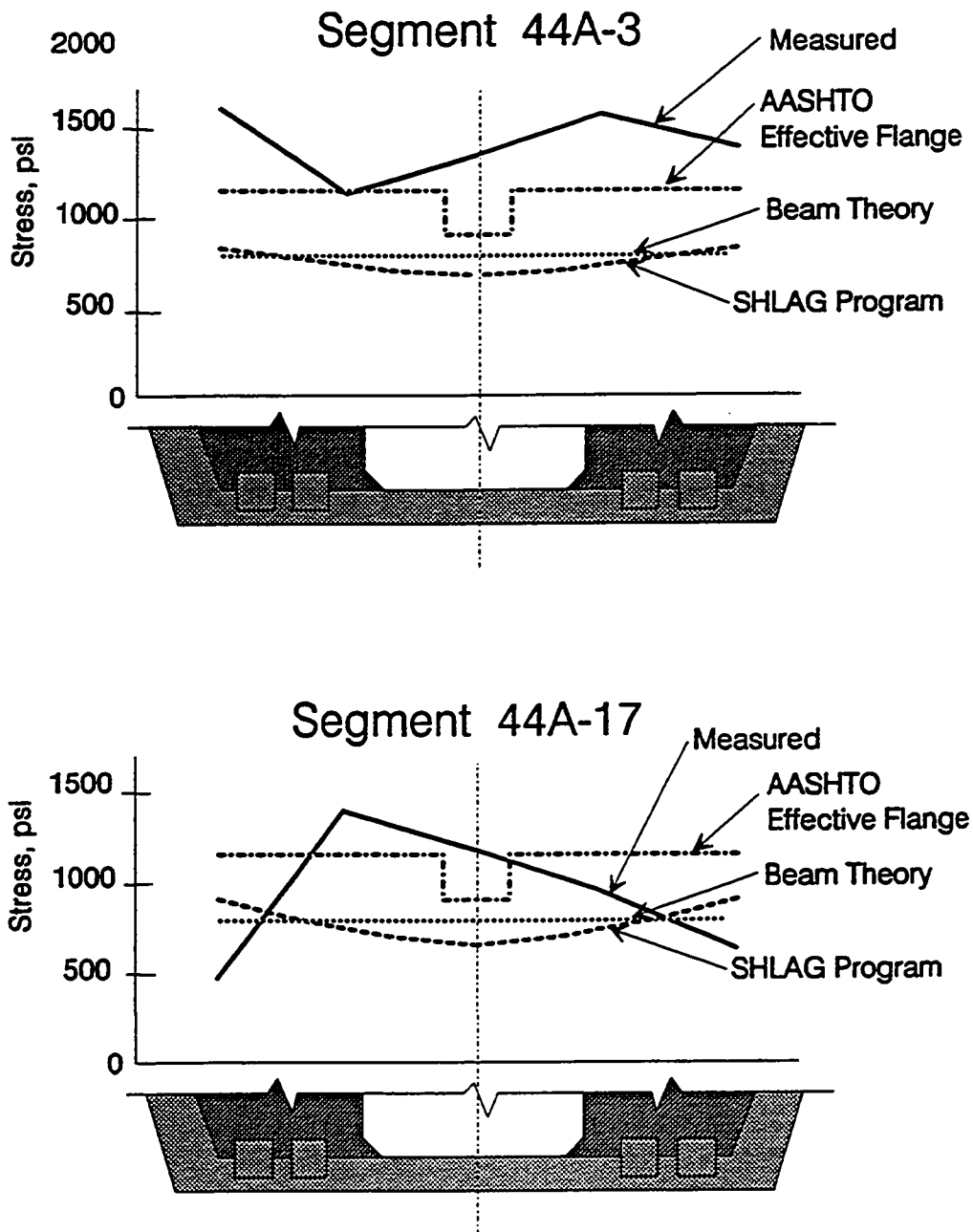
Figure 5.20 b) Bottom slab stress distributions, eleven feet from anchors.
