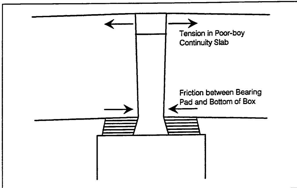
Figure 10.23 Continuity between spans C9 and C10.
