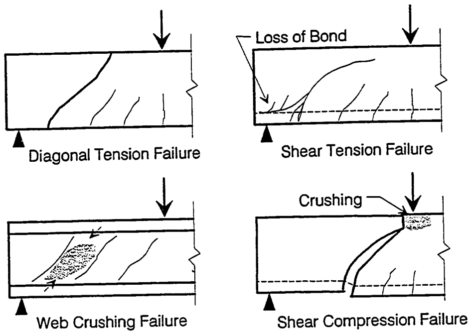
Figure 7.2 Shear failure modes for prestressed concrete beams.
