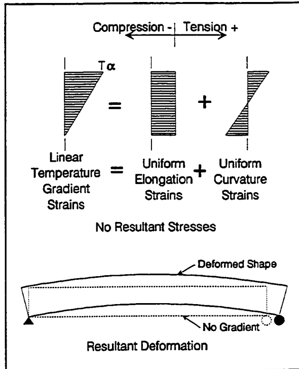
Figure 6.2 Determinant beam subjected to linear gradient.
