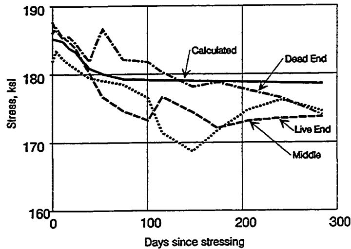
Figure 4.30 Adjusted average tendon stresses for Tendons T2N and T2S in Span A44.
