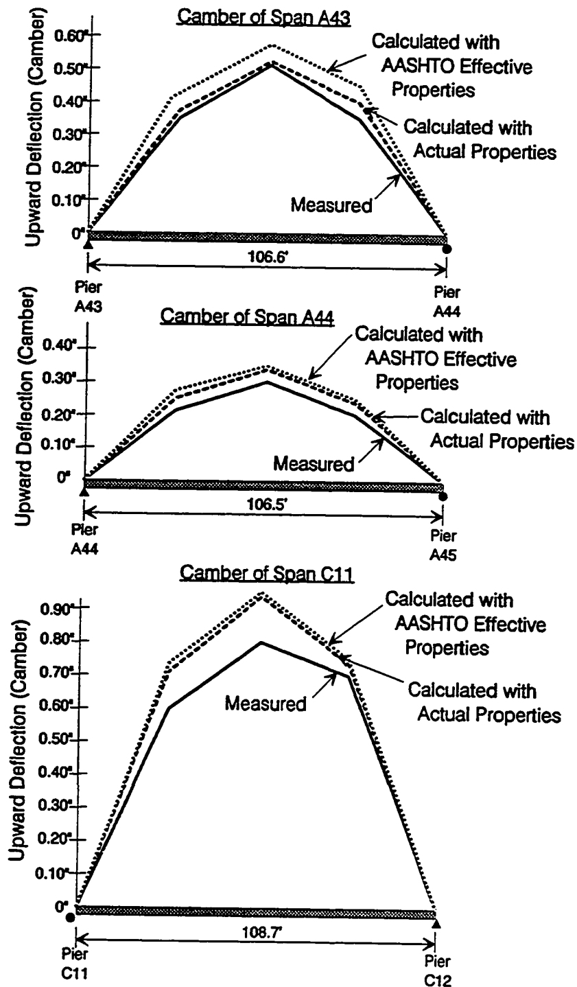
Figure 5.26 Comparison of actual and calculated span deflections (dead load and simple span tendons only).
