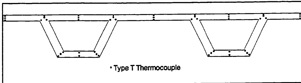
Figure 6.8 James River Bridge thermocouple layout.
