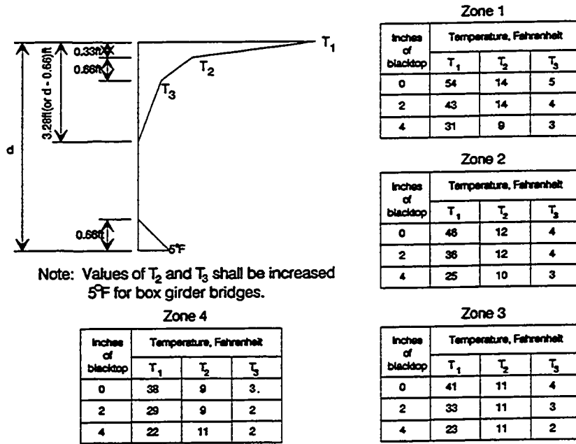
Figure 6.14 a) Design positive thermal gradients.
