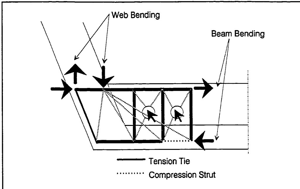
Figure 9.11 Strut-and-tie model for Span C11 deviator.
