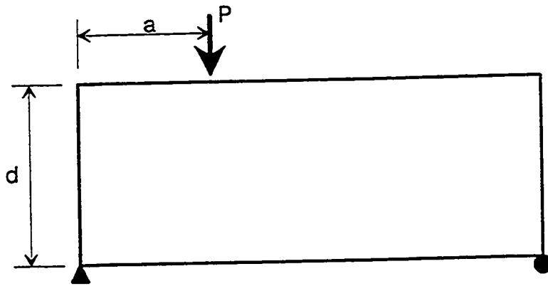
Figure 7.1 Definition of a/d ratio.
