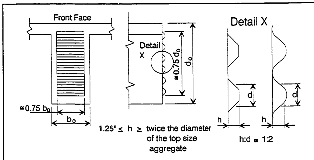
Figure 7.4 Figure 25-1 from AASHTO Guide Specification. Example of fine indentation joint faces.
