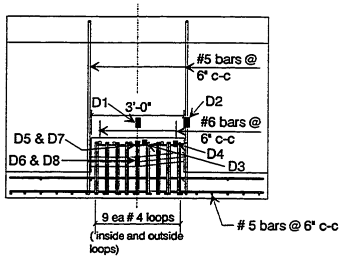
Segment 11C-5 Section View
