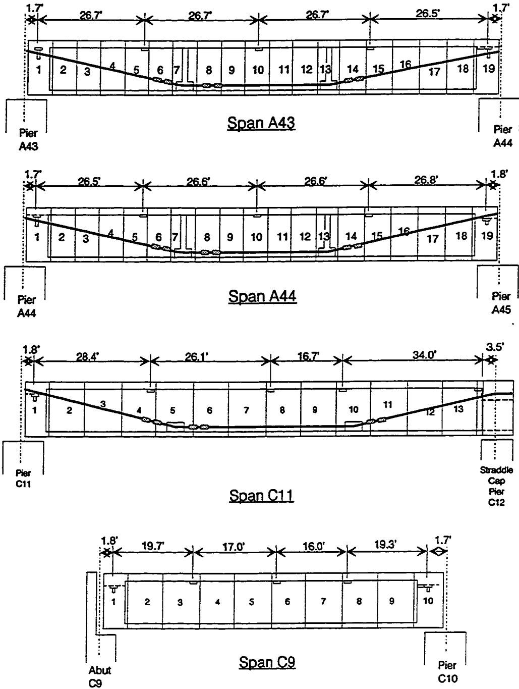
Figure 3.18 Deflection measurement system layouts.
