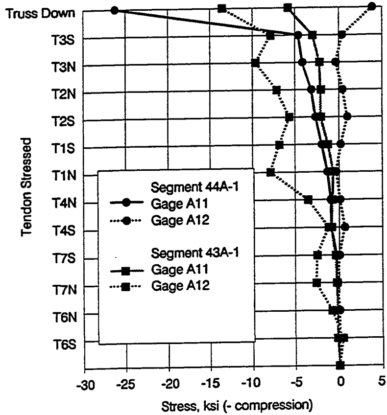
Figure 8.15 Stresses in top and bottom slab bars.
