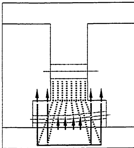
Figure 9.14 Section view of strut-and-tie model for spans A43 and A44 deviators.
