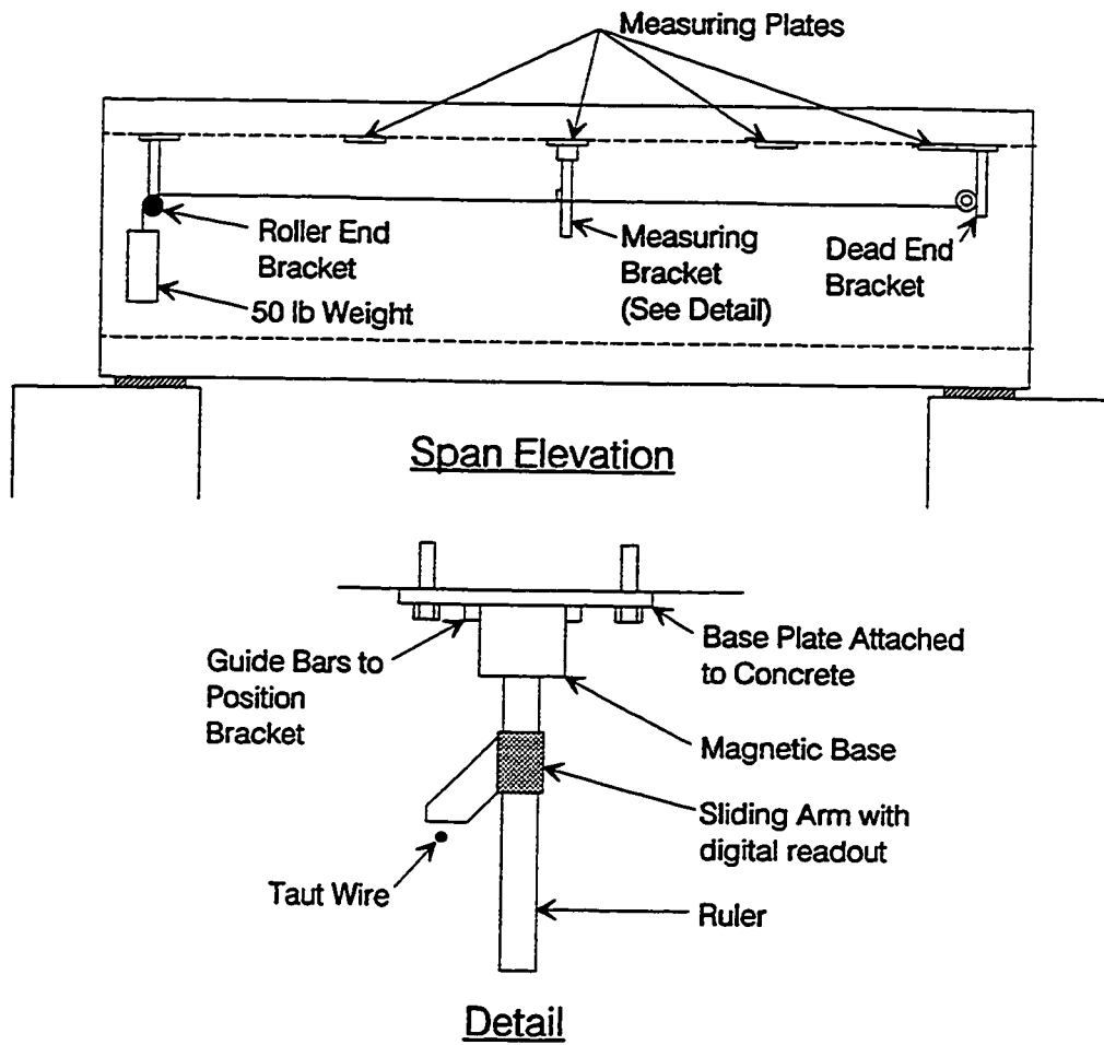
Figure 3.17 Taut wire baseline system.
