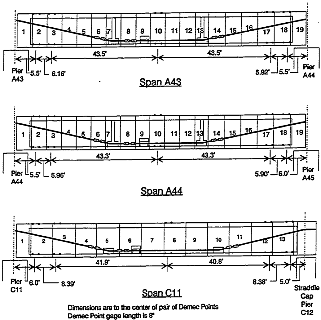
Figure 3.16 b) Demec point layouts.
