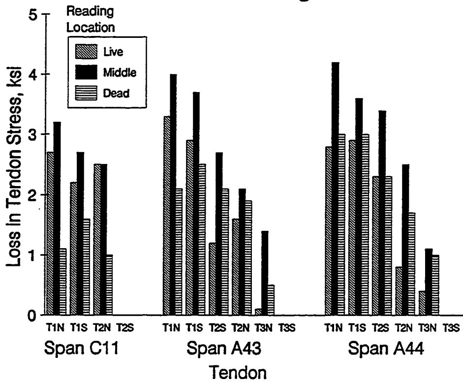
Figure 4.17 Elastic shortening losses.
