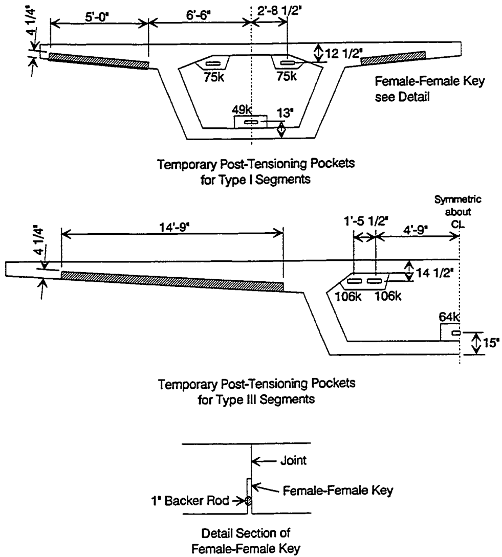
Figure 7.12 Temporary post-tensioning details.
