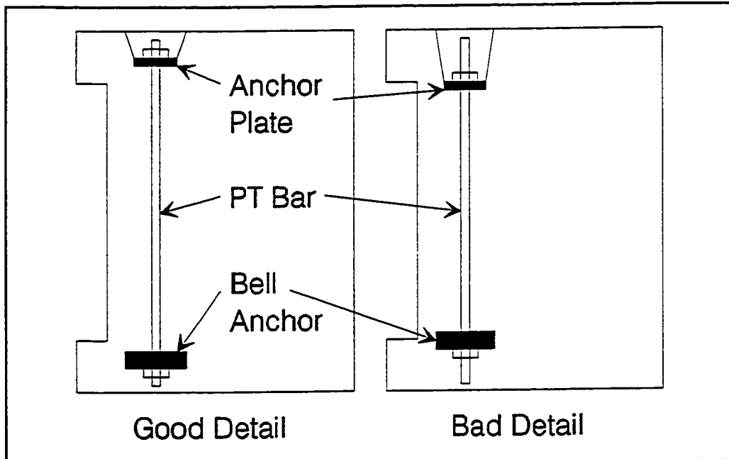
Figure 8.26 Comparison of well anchored and inadequately anchored vertical post-tensioning bar.
