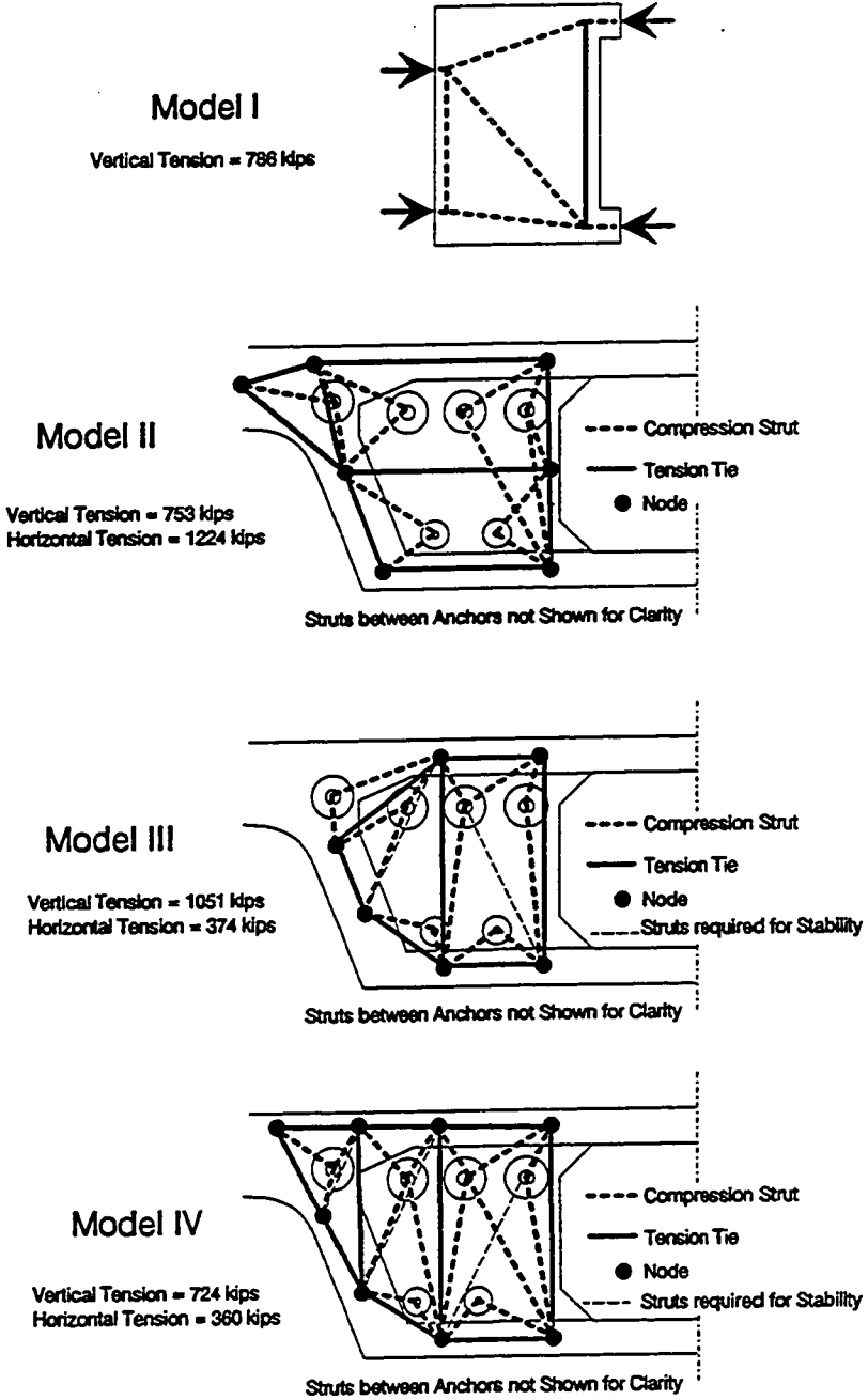
Figure 8.20 Strut-and-tie models for diaphragm.
