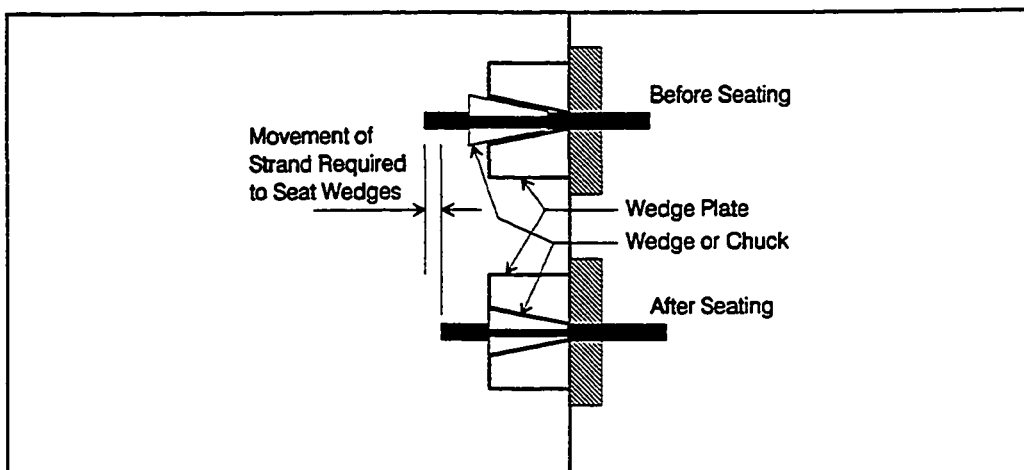
Figure 4.6 Movement of strand during seating of wedges.
