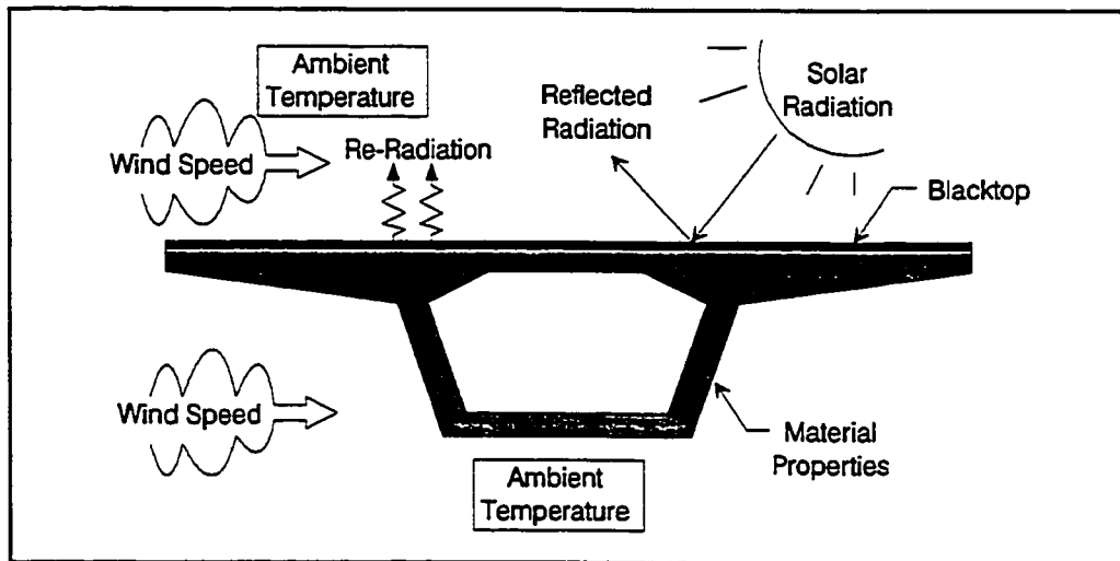
Figure 6.1 Factors affecting thermal gradient.
