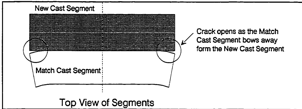
Figure 11.9 Cracks indicate joint opening.
