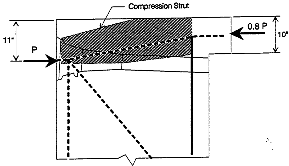
Compression Strut in Expansion Joint Segment
