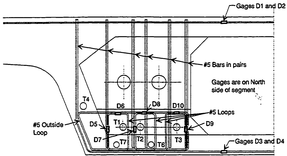
Span A43 and A44 Deviator Segment Elevation View
