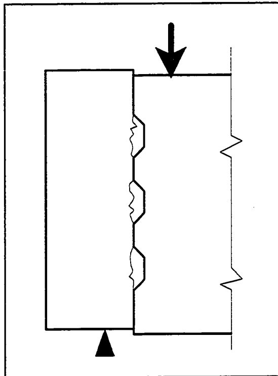
Figure 7.3 Joint shear failure.
