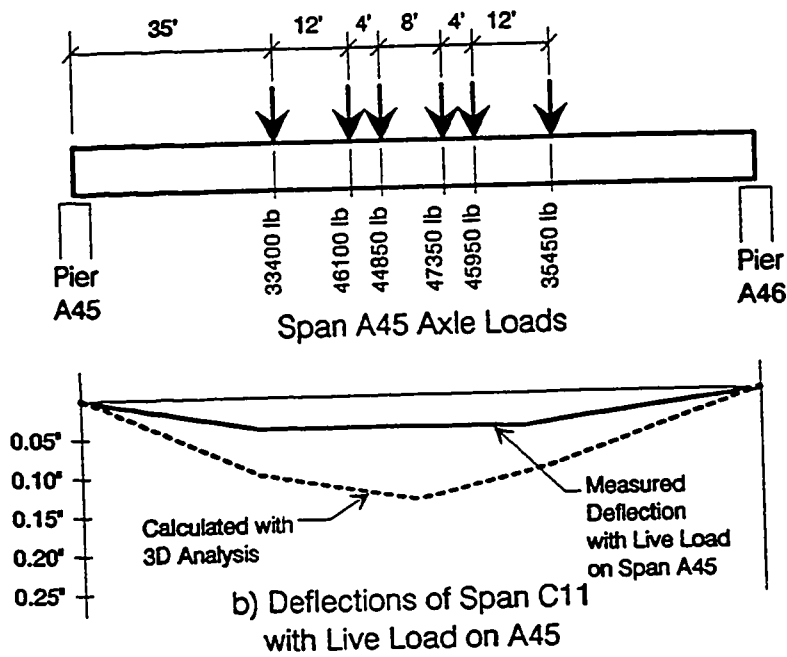
Figure 10.24 Calculated vs. actual deflections of span C11 with live loads.
