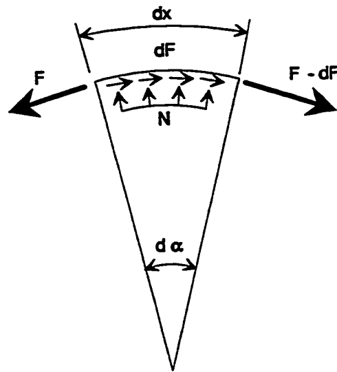
Figure 4.3 Friction loss along length dx .
