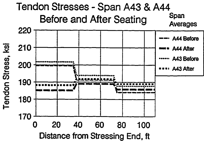
Figure 4.16 Losses in tendon stress due to seating.
