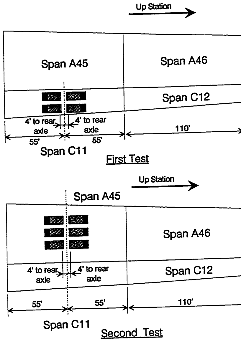
Figure 10.11 Truck positions in spans C11 and A45.
