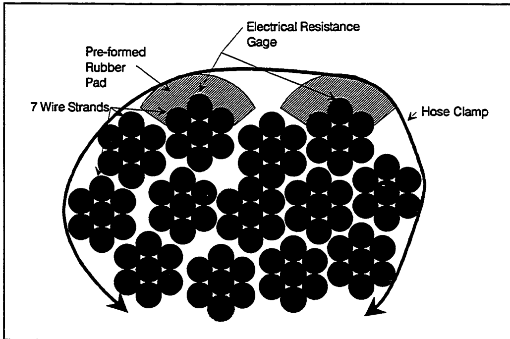
Figure 3.9 Clamping system for ER gages on tendon bundles.
