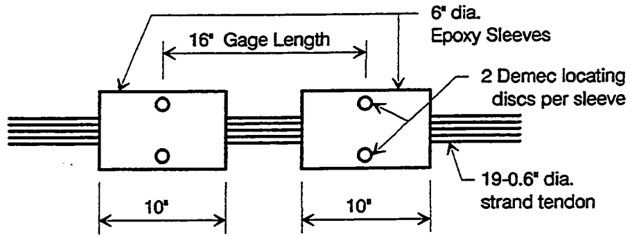
Figure 3.4 Schematic of epoxy sleeve system.
