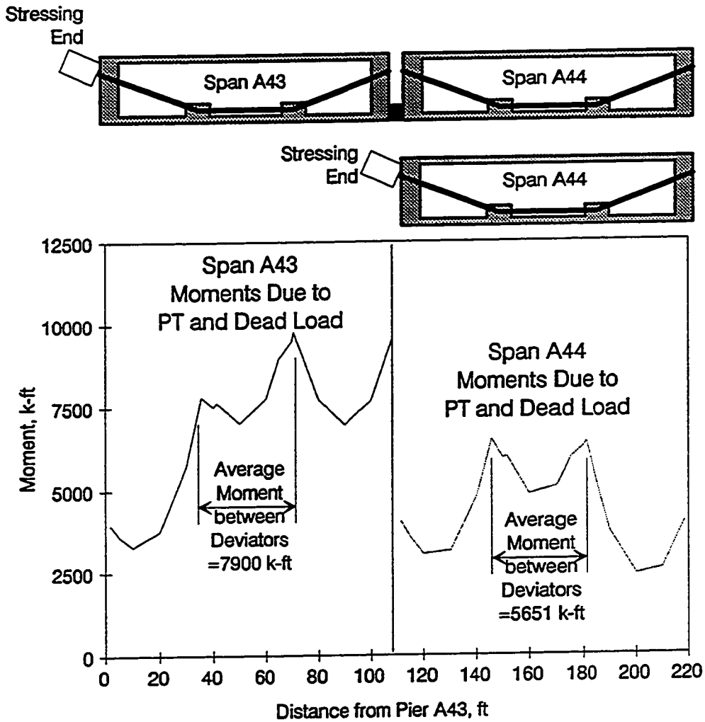
Figure 4.19 Moments between deviators.
