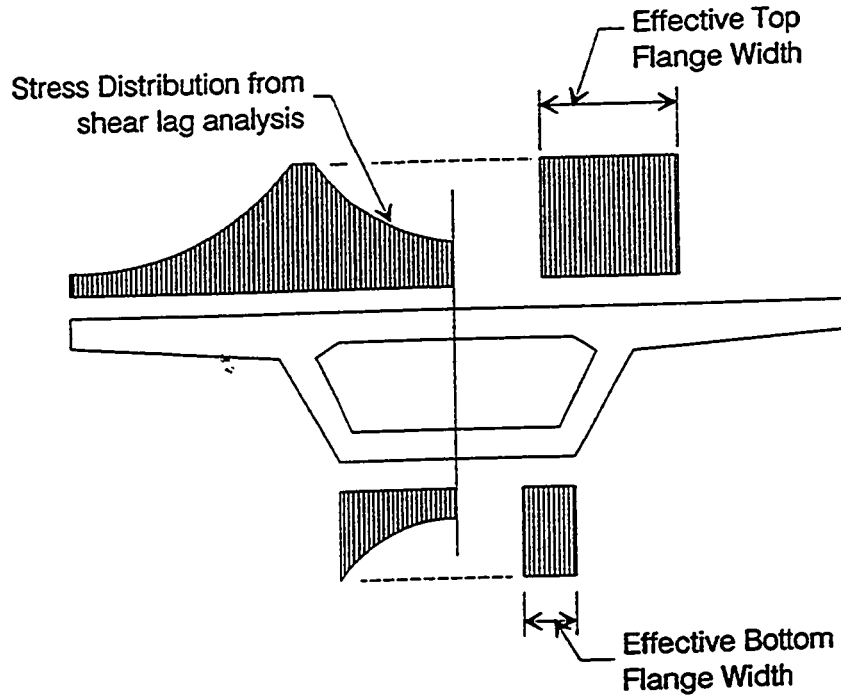
Figure 5.3 Definition of effective flange width.
