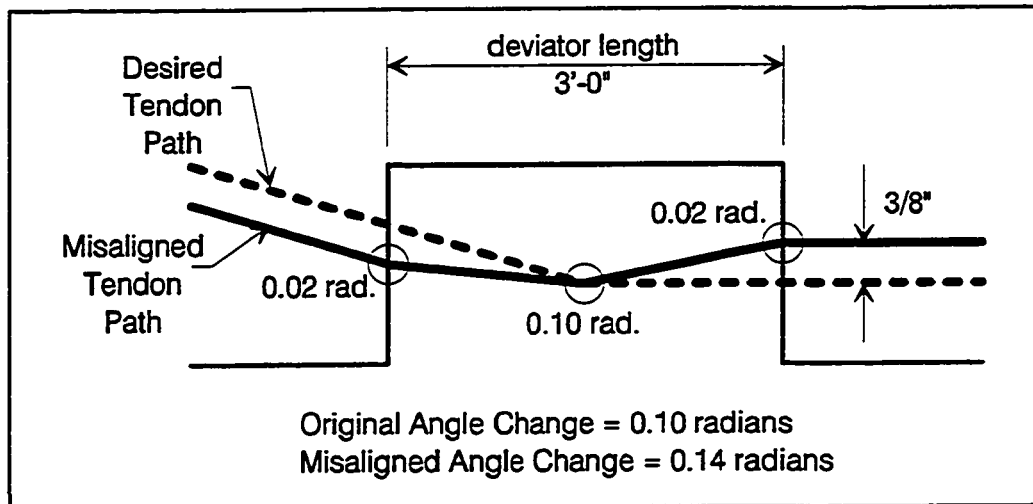
Figure 4.14 Effect of deviator duct misalignment.
