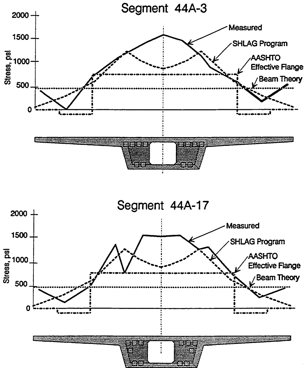
Figure 5.17 b) Top slab stress distributions, eleven feet from anchors.
