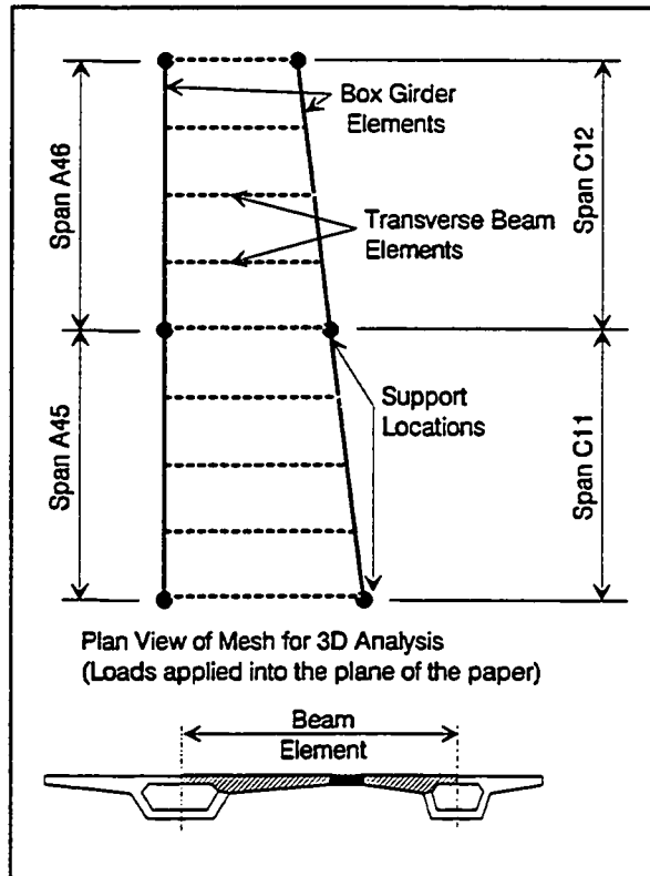
Figure 10.25 Model of spans A45 and C11.
