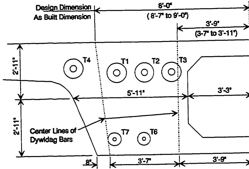
Dywidag Bar Locations - Elevation View
