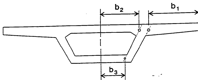
Figure 5.4 Flange widths as defined by the AASHTO Guide Specification .
