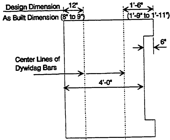
Dywidag Bar Locations - Section View
