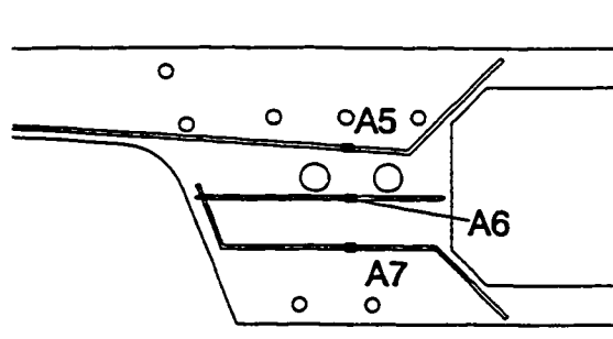
Stresses in Horizontal Reinforcing Bars In Diaphragm Segments
