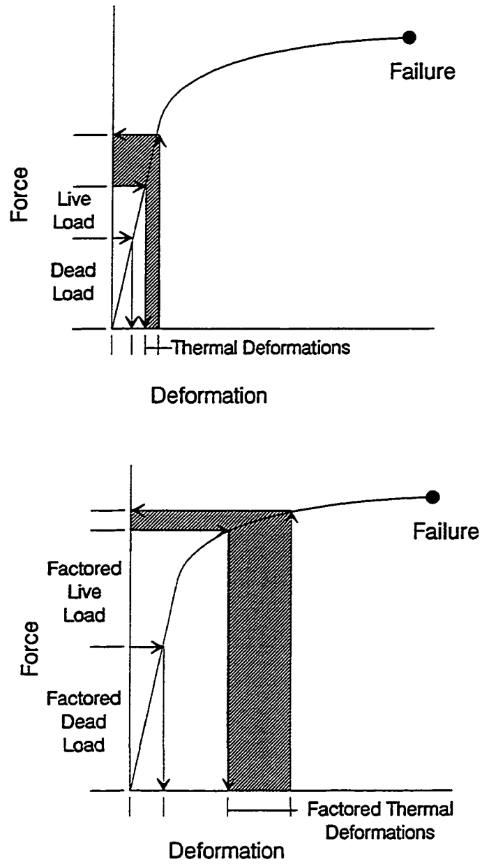
Figure 6.11 Comparison of thermal effects at service and ultimate loads.
