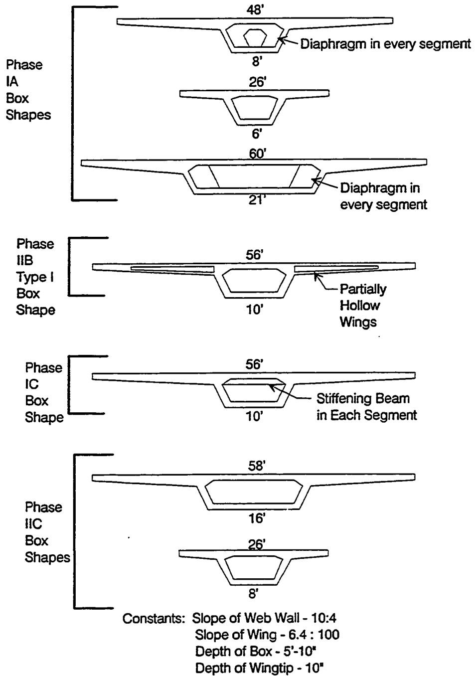
Figure 2.5 Sample box shapes from previous and current phases of the San Antonio "Y" Project.
