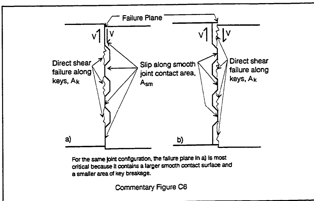
Figure 12.3 Joint shear failure plane.
