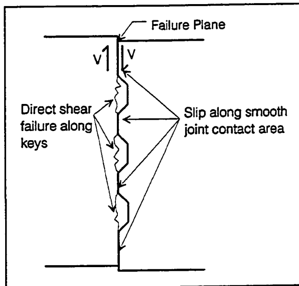
Figure 7.19 Joint shear failure plane.
