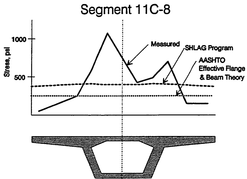
Figure 5.18 b) Top slab stress distribution, at mid-span.
