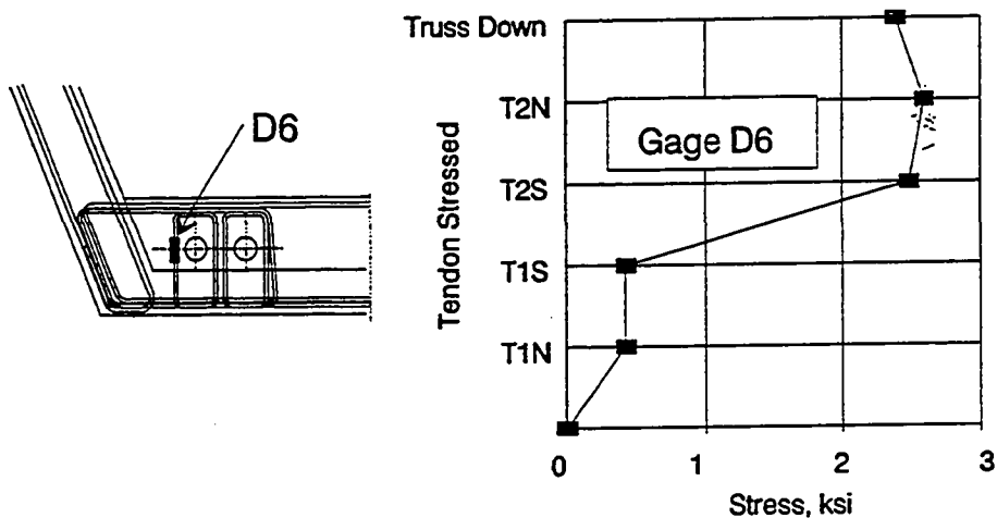
Figure 9.7 Stresses in vertical bars.
