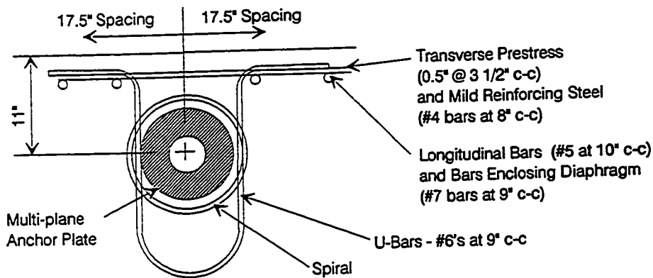
Anchorage Device and Reinforcing as Designed in Expansion Joint Segments
