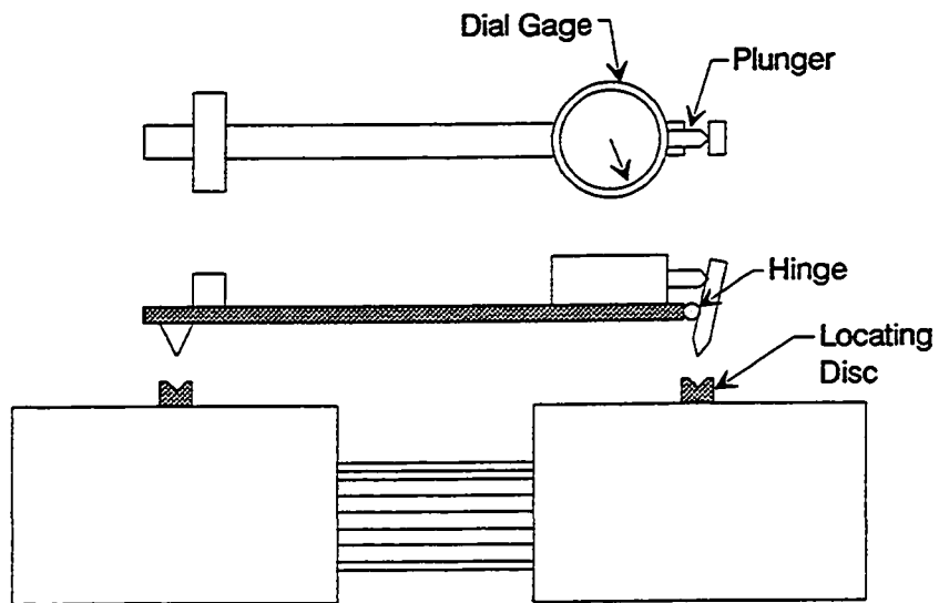
Figure 3.5 Demec extensometer.
