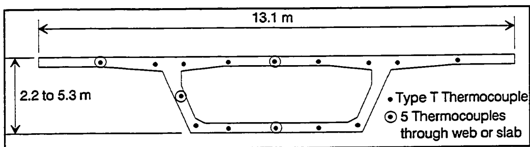
Figure 6.7 Red River Bridge thermocouple layout.
