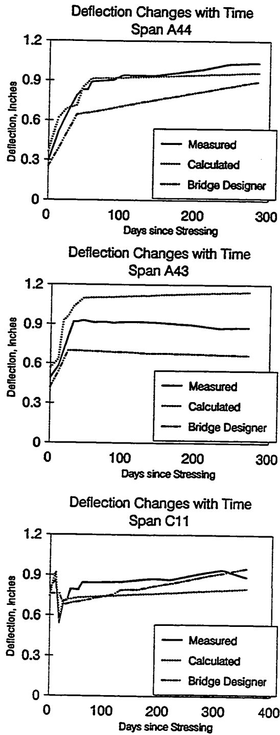
Figure 4.22 Comparison of measured and calculated deflection.
