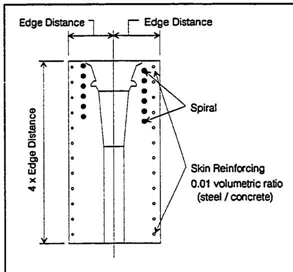
Figure 8.23 Dimensions of local zone test block.
