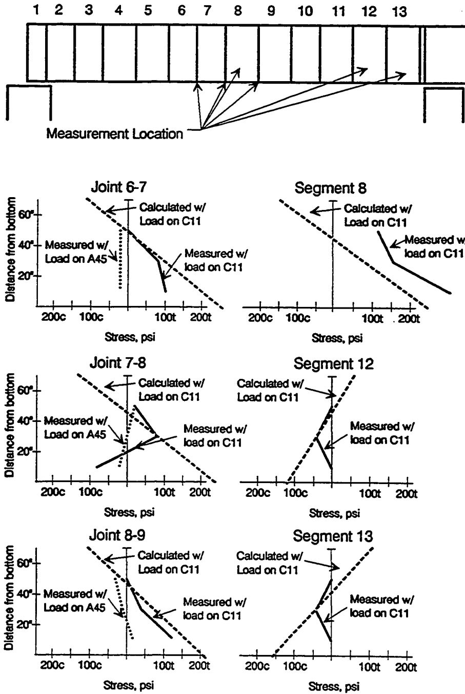
Figure 10.28 Web stress profiles in span C11.
