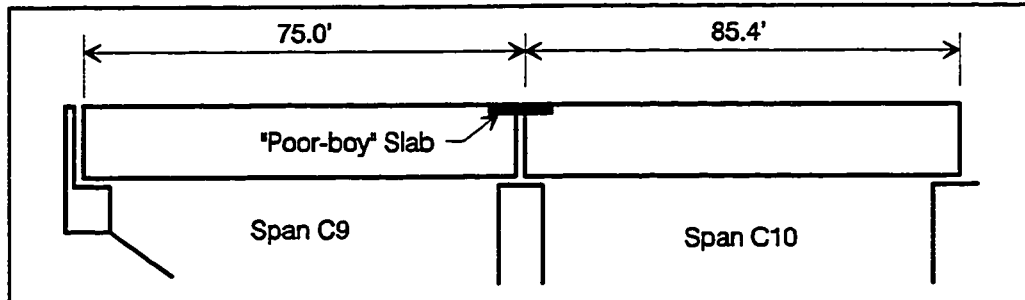
Figure 1.4 "Poor-boy" continuity.
