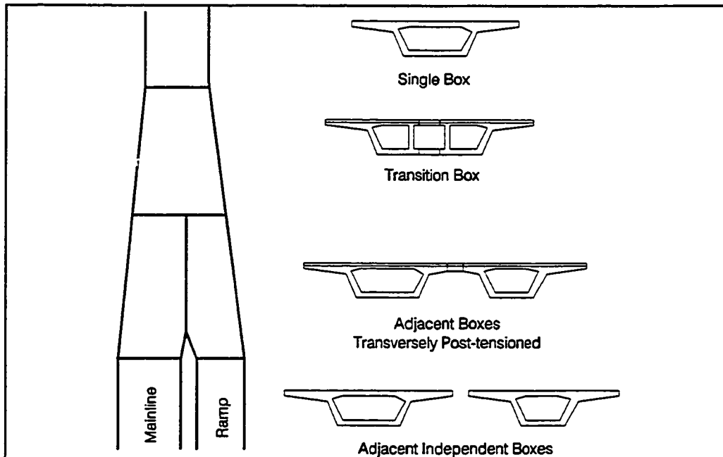
Figure 10.4 Ramp box merging with mainline box.
