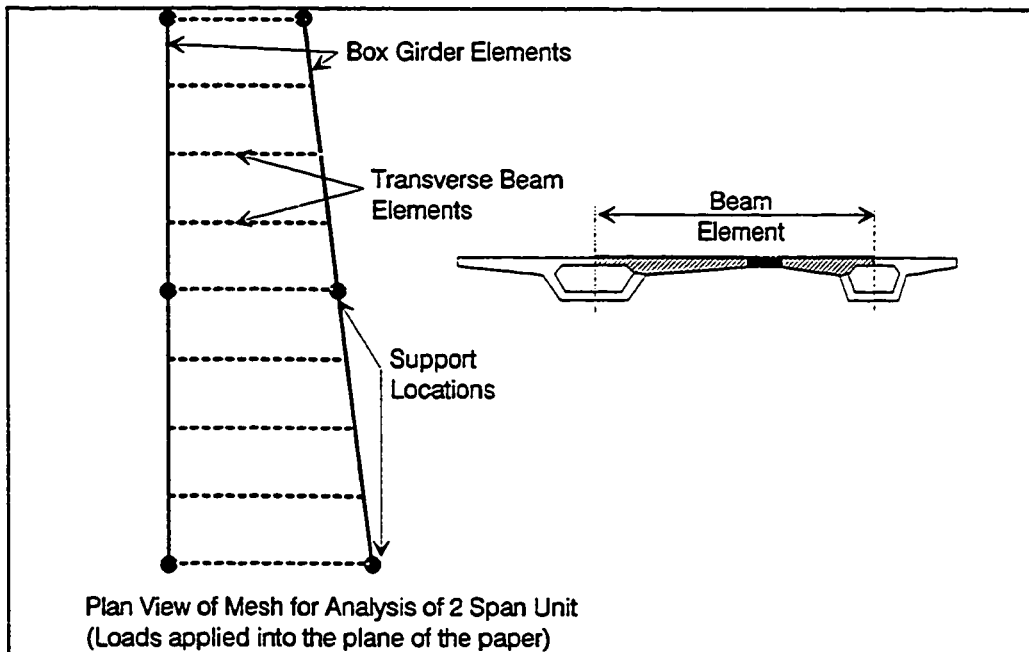
Figure 12.5 Model of transversely post-tensioned box girders.
