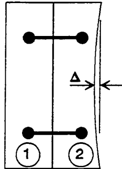
b) First two segments are epoxied and temporary post-tensioning is applied. Segments deform to close joint.
