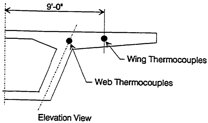
Figure 11.4 Typical thermocouple layout.
