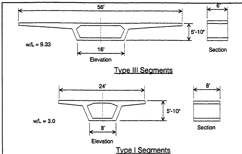
Figure 11.3 Segment types.
