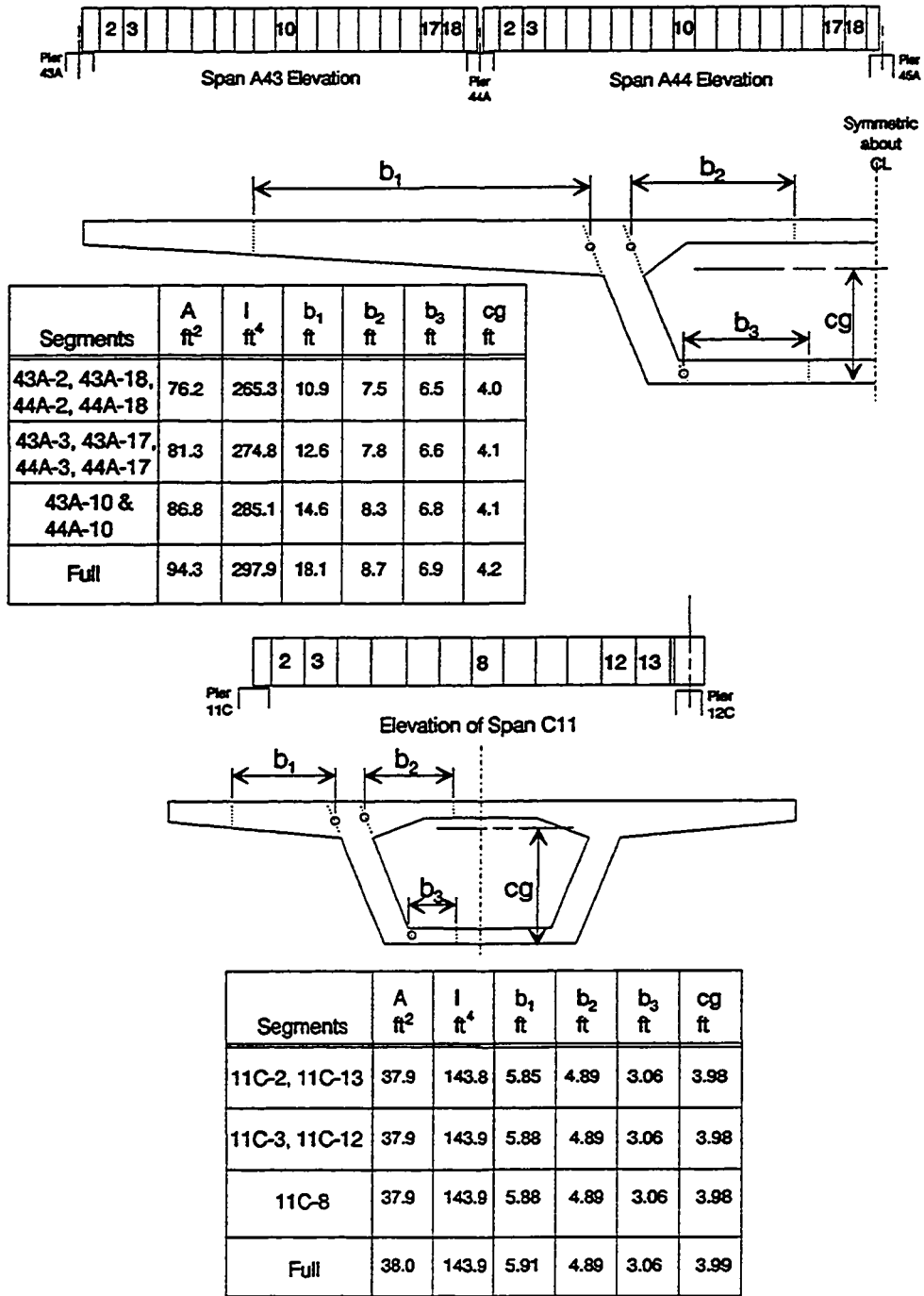
Figure 5.15 Effective segment properties per AASHTO.
