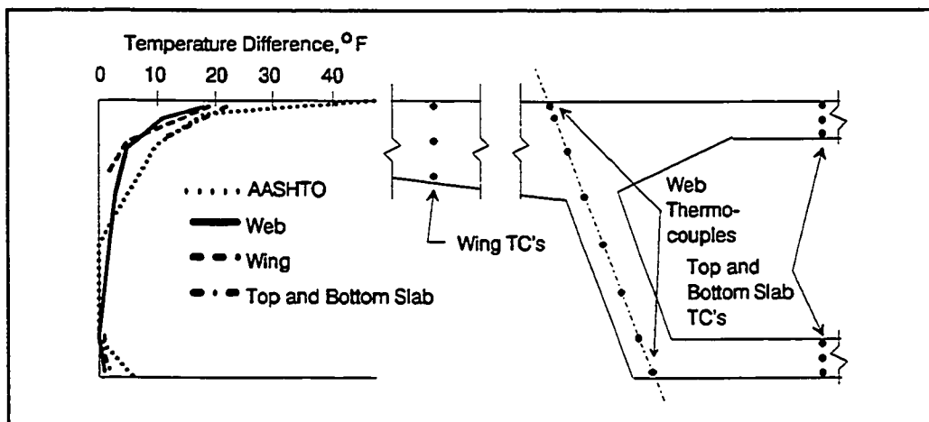
Figure 6.18 Comparison of wing, web and slab temperatures on July 16, 1992.
