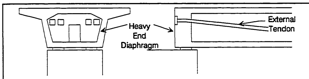
Figure 1.1 Heavy end diaphragm in segmental box girder with external tendons.
