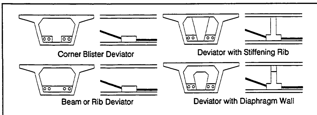
Figure 9.1 Deviator types.
