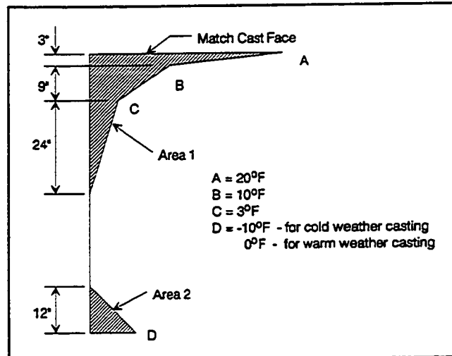
Figure 11.14 Design thermal gradient.
