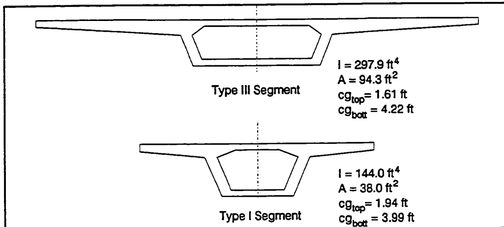
Figure 5.11 Segment properties.
