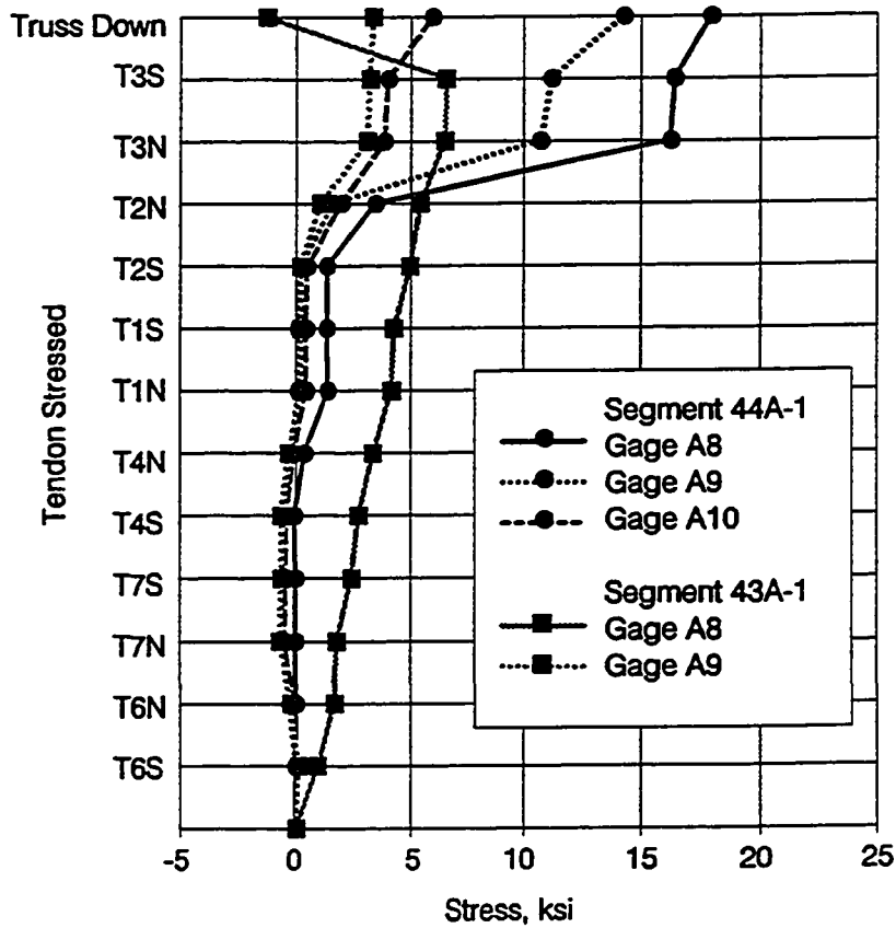
Figure 8.14 Stresses in U-shaped reinforcing bars.
