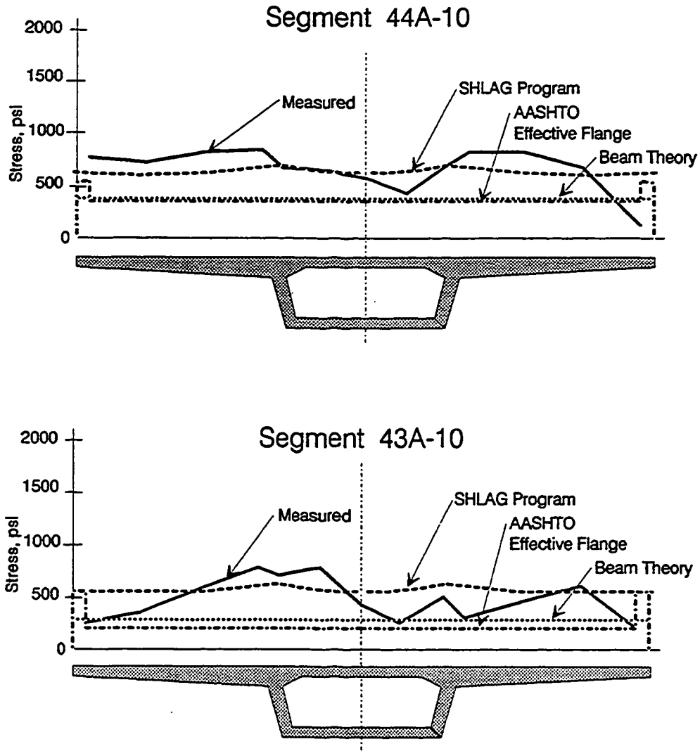
Figure 5.18 a) Top slab stress distributions, at mid-span.
