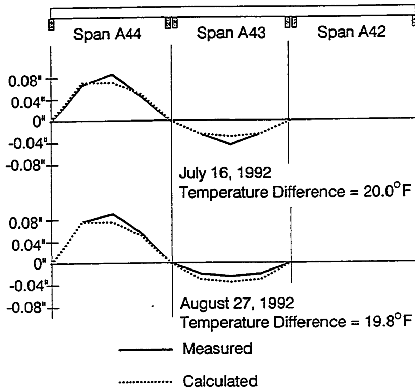
Figure 6.25 Measured and calculated deflections caused by thermal gradients.
