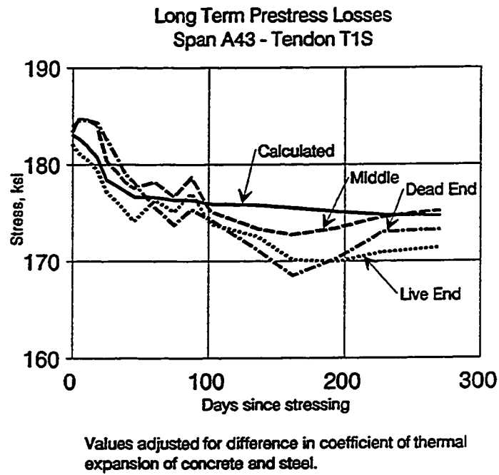
Figure 4.26 Adjusted average tendon stresses for Tendon T1S in Span A43.
