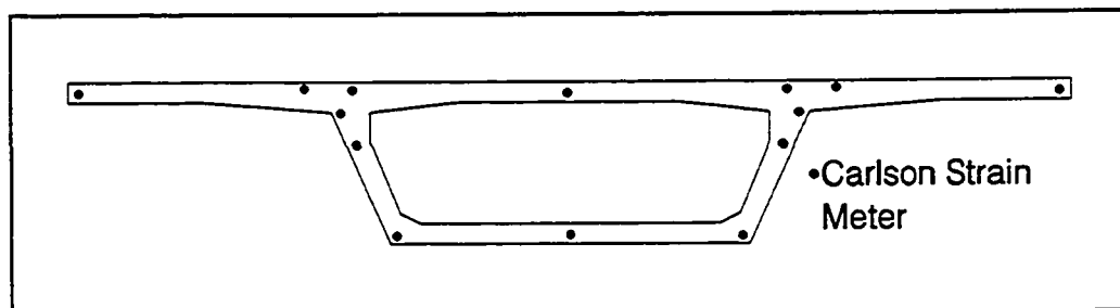
Figure 6.6 Denny Creek bridge Carlson gage layout.
