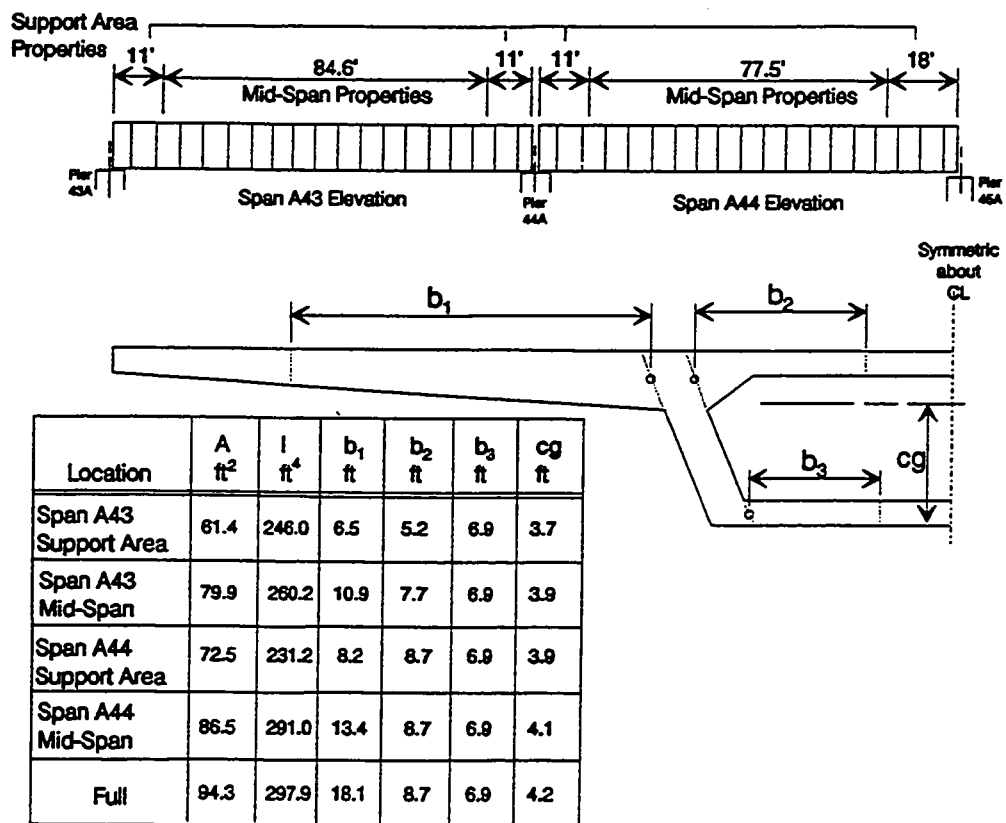
Figure 5.27 Effective segment properties using modified AASHTO method.
