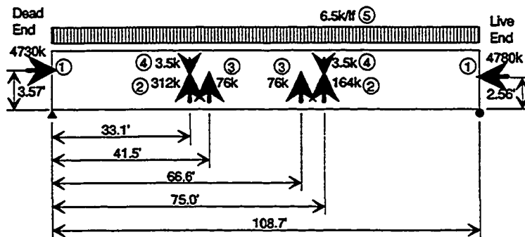
Span C11 Loading Diagram
