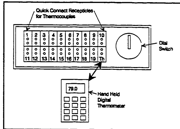
Figure 3.19 Thermocouple manual switchbox.
