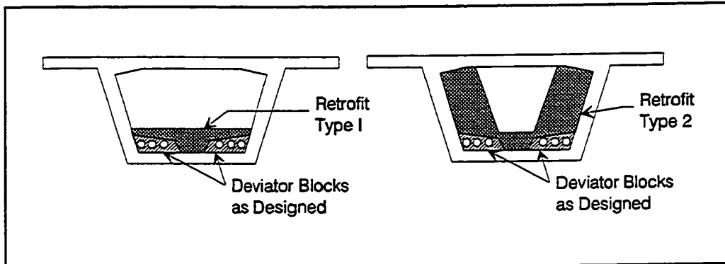
Figure 9.4 Retrofit to strengthen deviators.
