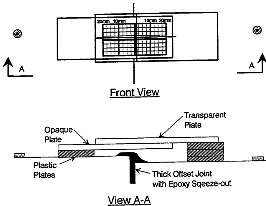
Figure 3.24 Grid crack monitor at offset joint.
